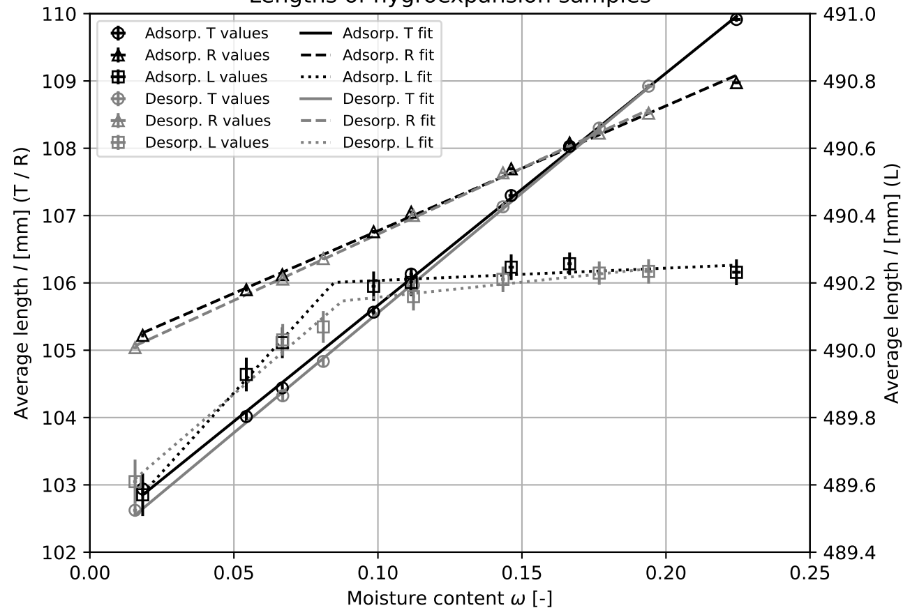
Lengths of hygroexpansion samples
