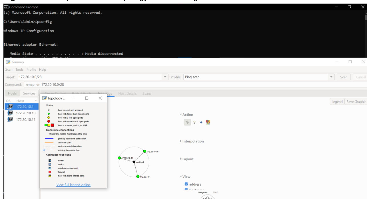
Figure 9: Zenmap – Network Topology view with legend enabled
