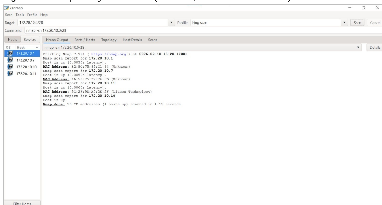
Figure 8: Zenmap – Ping Scan results (live hosts, IP and MAC addresses)
