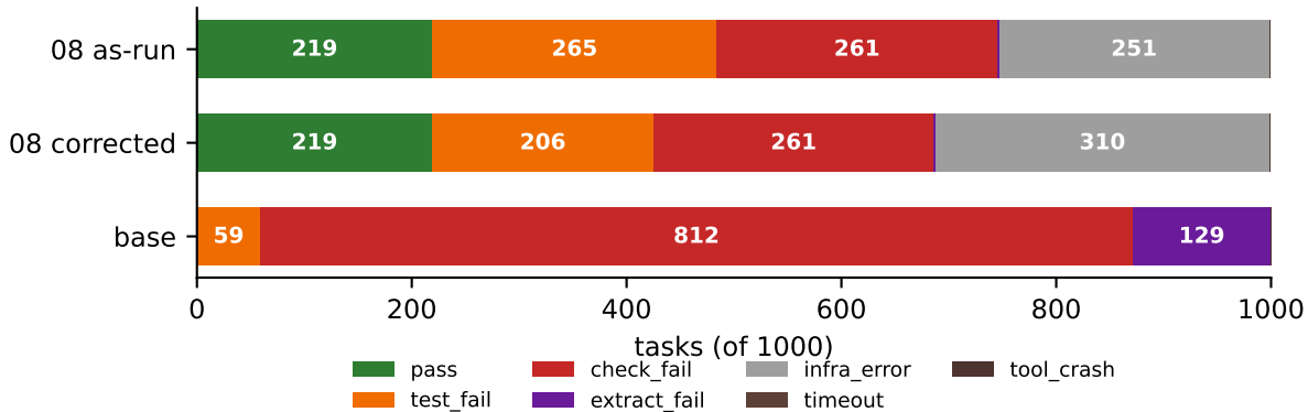
Grading outcome per task — 08 run is contaminated by disk-full infra failures
