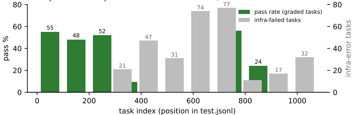
08 pass rate collapses in disk-affected windows; late blocks never recover
