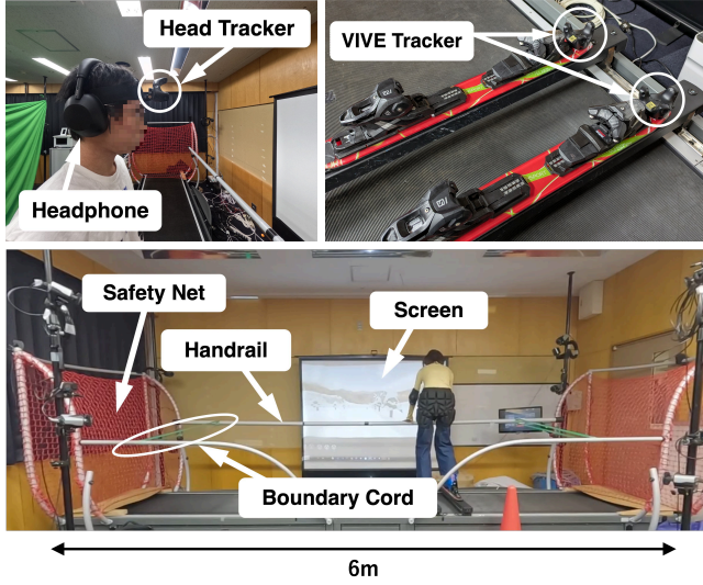
Figure 2: Hardware configuration of the simulator-based evaluation. VIVE trackers on the skis and head capture user motion and viewpoint, while headphones present spatial audio cues.
