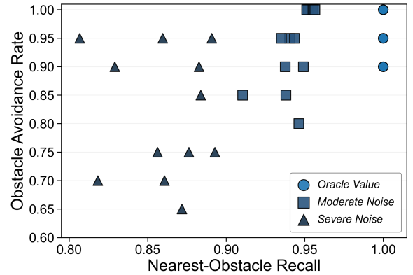
Figure 9: Results of Study 2 on the relationship between Nearest-Obstacle Recall and Obstacle Avoidance Rate. P06 was excluded from this analysis because the corresponding frame-level recordings were unavailable.
