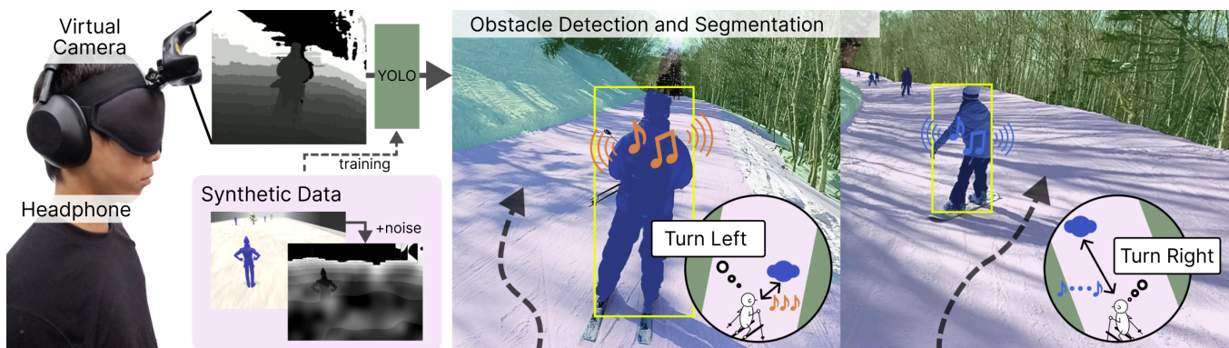
Figure 1: Overview of SnowEcho, an end-to-end blind skiing assistance system for simulated skiing. A head-mounted virtual camera captures the skier's viewpoint, and depth images augmented with real-slope-inspired noise are used for obstacle detection and segmentation. The system then renders spatial audio cues that convey obstacle direction and distance, while side cues indicate course boundaries. Rather than prescribing a single avoidance route, SnowEcho externalizes surrounding hazards so that skiers can perceive traversable space and choose their own line.
