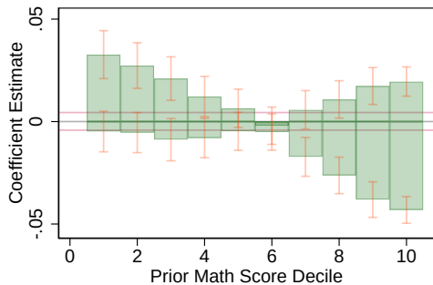
2-Year Enrollment on ELA and Math VA interacted with w/ prior Math Score Decile
