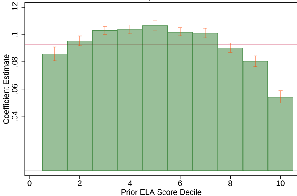
2-Year Enrollment on 2-Year Enrollment DK VA (without peer controls) interacted with w/ prior ELA Score Decile base sample and base controls
