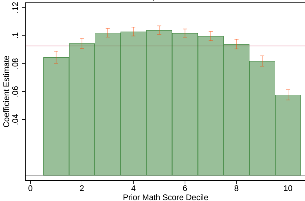
2-Year Enrollment on 2-Year Enrollment DK VA (without peer controls) interacted with w/ prior Math Score Decile base sample and base controls
