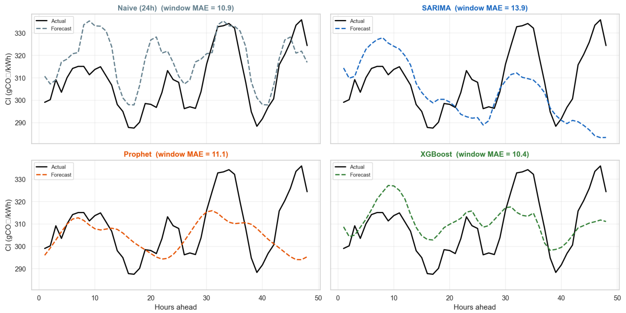
Figure 8.5 Example 48-hour forecasts from each model against the actual carbon intensity for one test window.
