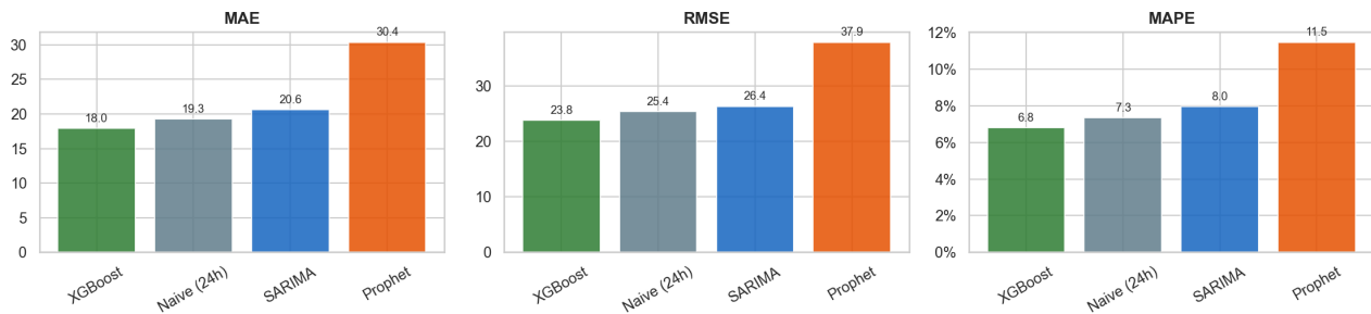
Figure 8.2 Model comparison across MAE, RMSE and MAPE. XGBoost is the only model to beat the naive baseline on all three metrics.
