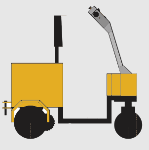
STANDING TOW TRUCK Capacity: 1-3 Ton Turning Radius: 1.5 Mtr Battery: LFP Overall Size: 1500x750x1180mm
