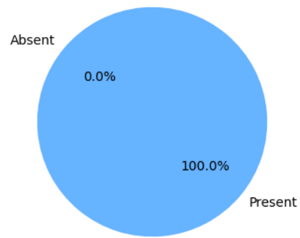
Attendance Distribution in BCS403
