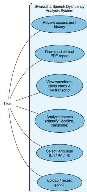
Figure 3.3: Use Case Diagram
