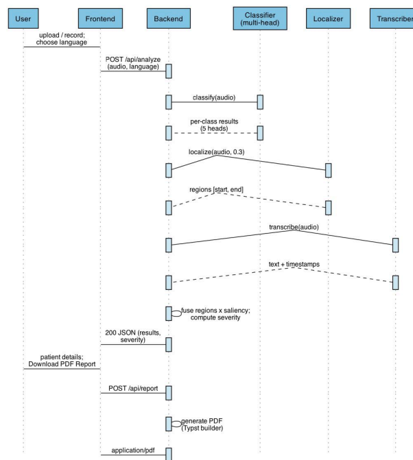
Figure 3.5: Sequence Diagram
