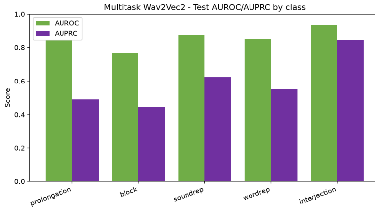
Fig. 3. Per-class AUROC and AUPRC (multitask Wav2Vec2) on the clip-level test set.
