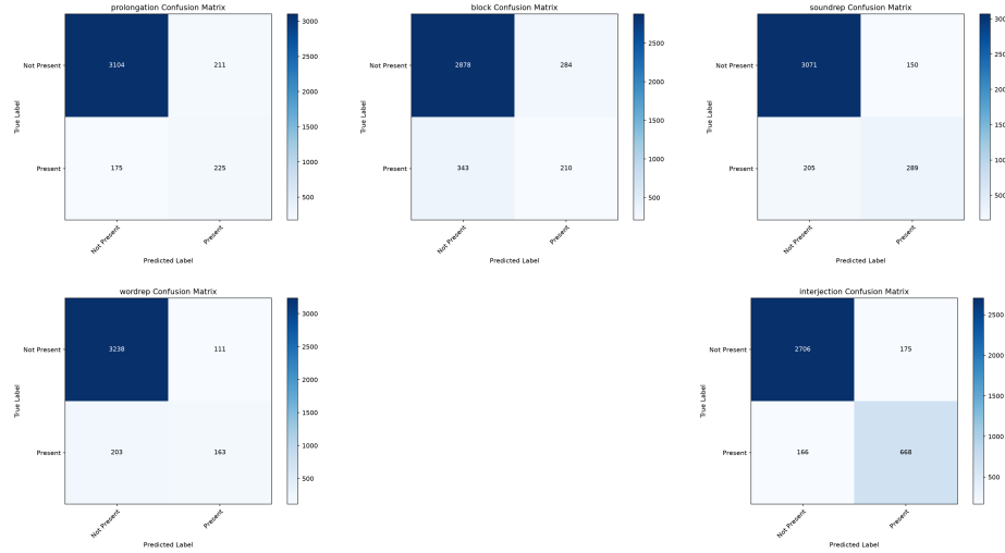
Fig. 4. Confusion matrices for the five binary Wav2Vec2 classifiers (arm01) on the clip-level in-distribution test set. Top row: prolongation, block, and sound repetition; bottom row: word repetition and interjection.
