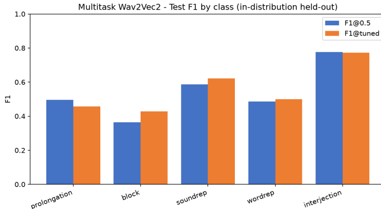
Fig. 1. Per-class F1 scores (multitask Wav2Vec2) on the clip-level in-distribution test set.
