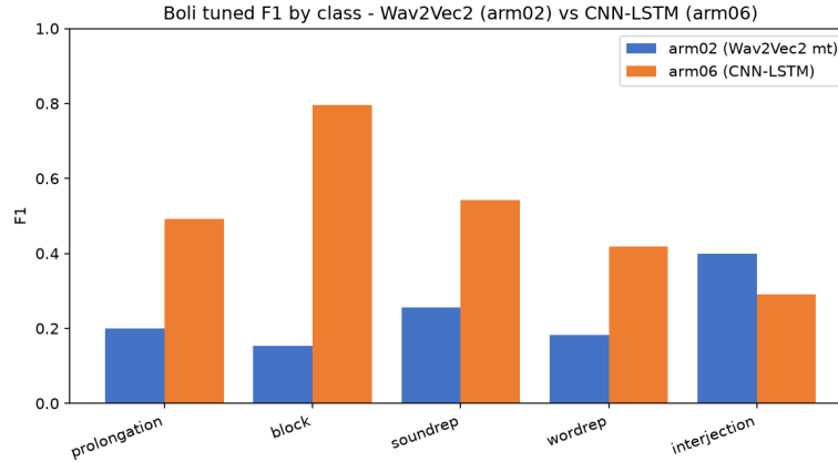
Fig. 2. Per-class tuned F1 on the Project Boli speaker-independent cross-corpus set for the shared-backbone Wav2Vec2 model (arm02) and the CNN-LSTM model (arm06), each using its per-class validation-F1-optimal thresholds.
