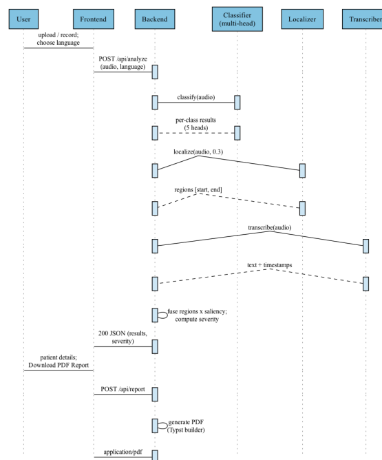
Figure 3.5: Sequence Diagram
