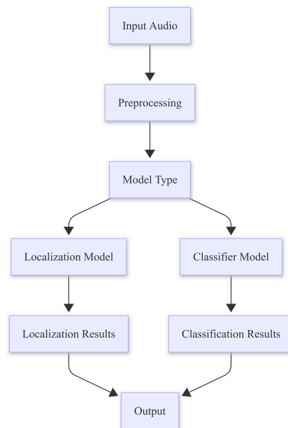
Figure 3.1: System Architecture
