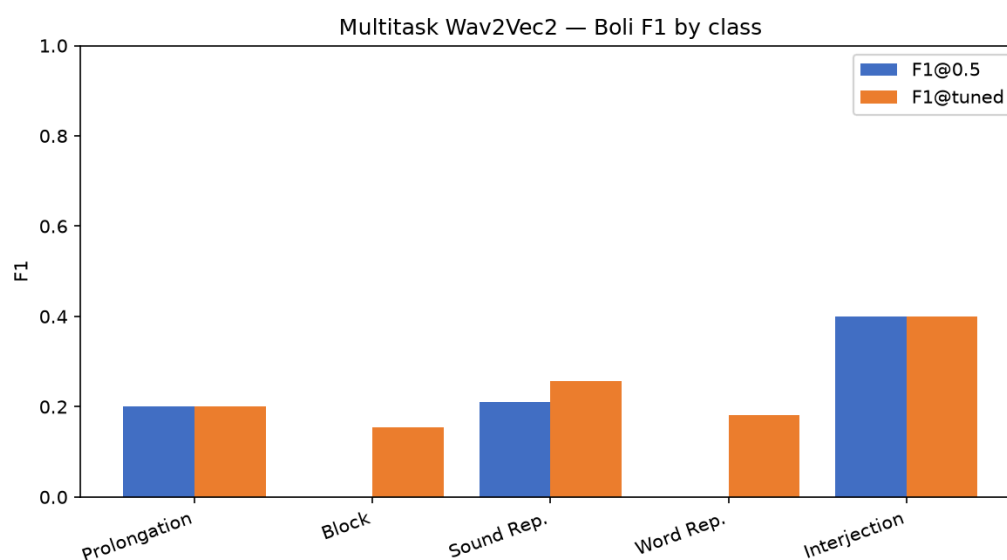
Figure 5.5: Per-class tuned F1 on the Boli set
