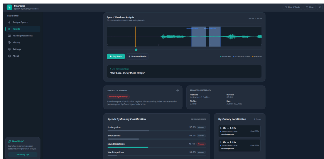
Figure 6.2: Results page of the web interface
