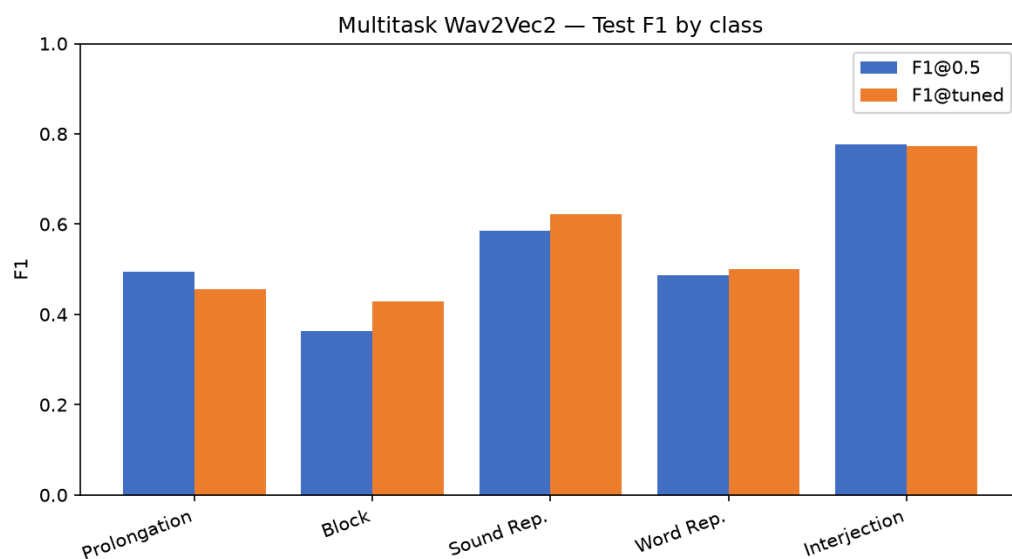
Figure 5.1: Per-class F1 of the multitask Wav2Vec2 classifier
