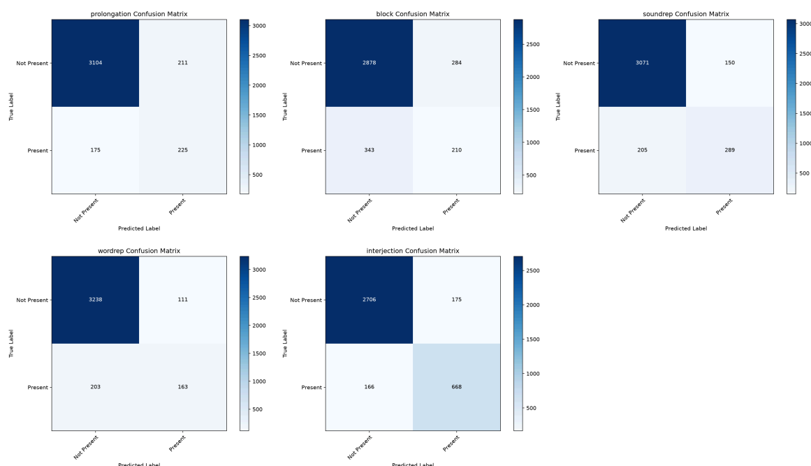
Figure 5.3: Confusion matrices for the five binary classifiers
