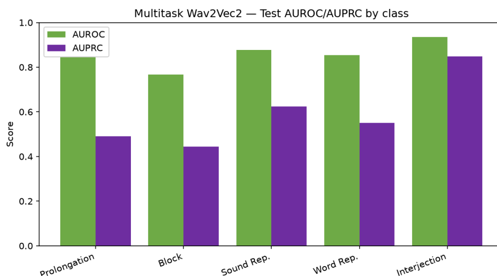
Figure 5.2: Per-class AUROC and AUPRC of the multitask Wav2Vec2 classifier
