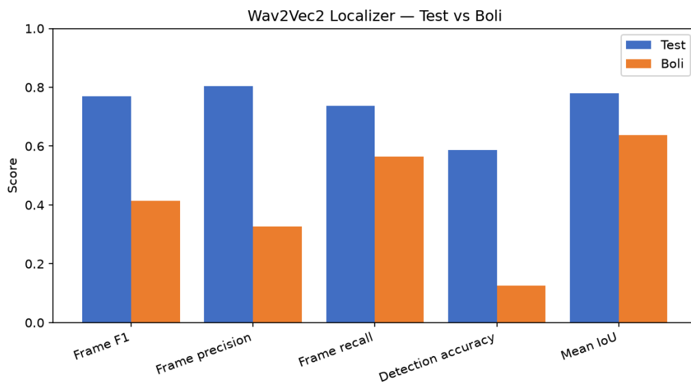
Figure 5.4: Frame-level metrics of the Wav2Vec2 localizer
