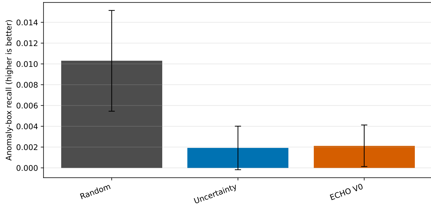
Final anomaly_recall (mean \pm 95% CI)
