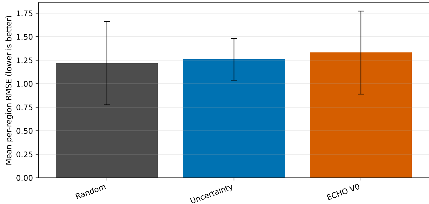
Final mean_region_rmse (mean \pm 95% CI)
