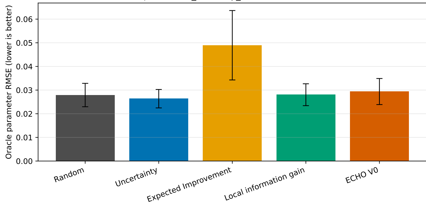
Final parameter_recovery_rmse (mean \pm 95% CI)
