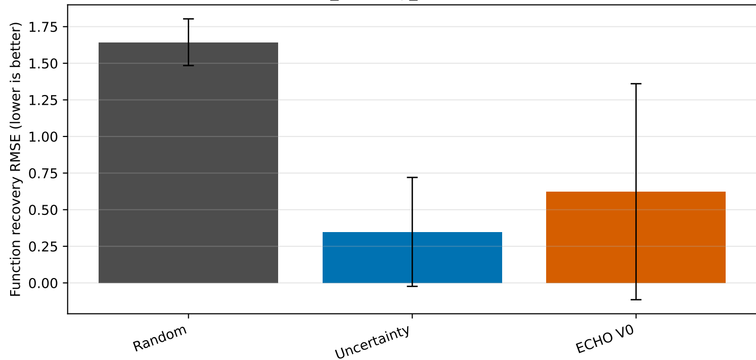
Final function_recovery_rmse (mean \pm 95% CI)
