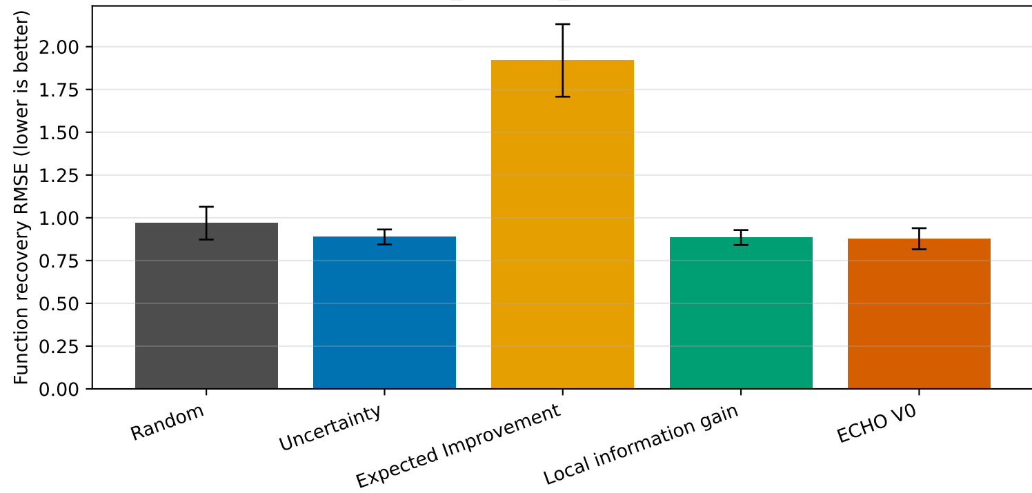
Final function_recovery_rmse (mean \pm 95% CI)
