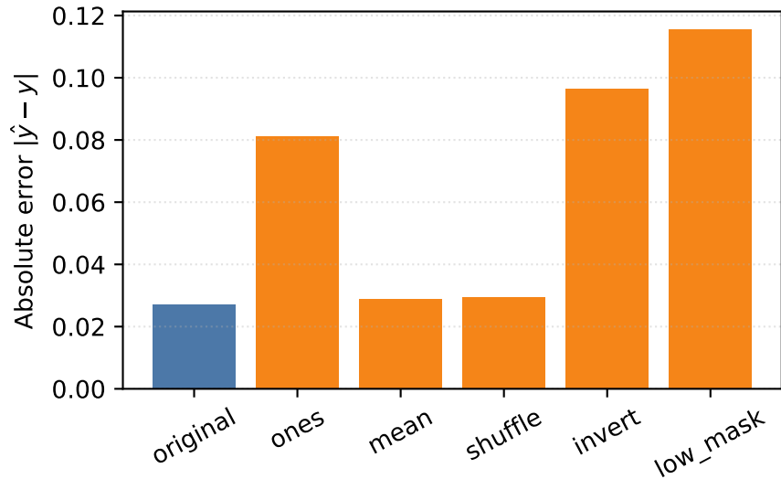
Error after confidence intervention
