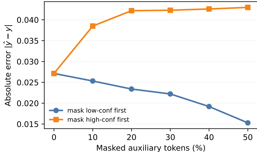
Error sensitivity
