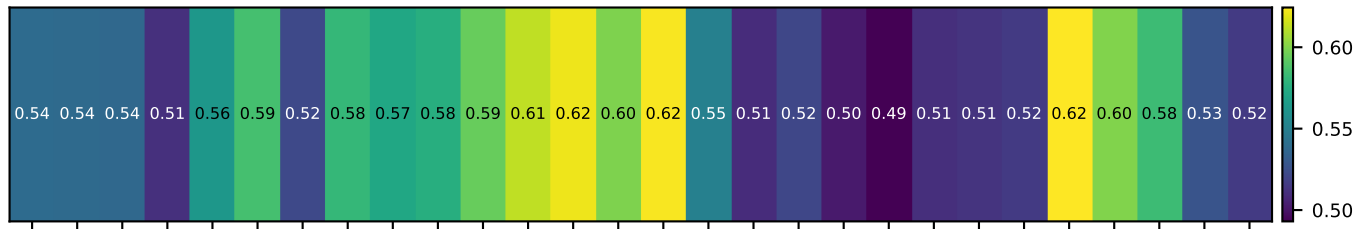
Token confidence and prediction sensitivity (original order)
