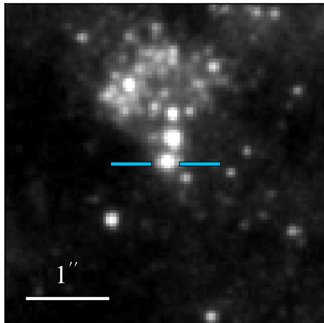
WFC3 F475W: 22.372 \pm 0.007
