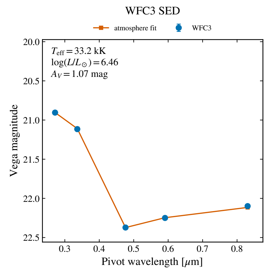
WFC3 F814W: 22.099 \pm 0.012
