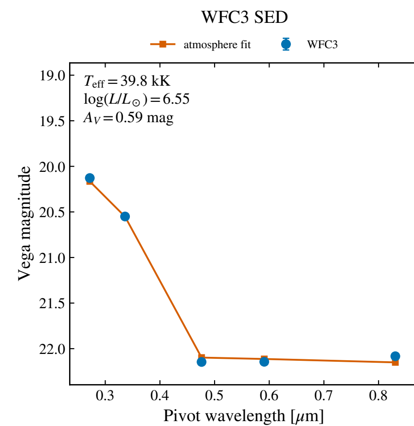
WFC3 F814W: 22.083 \pm 0.013
