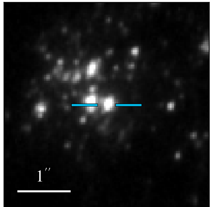
WFC3 F275W: 18.544 \pm 0.007
