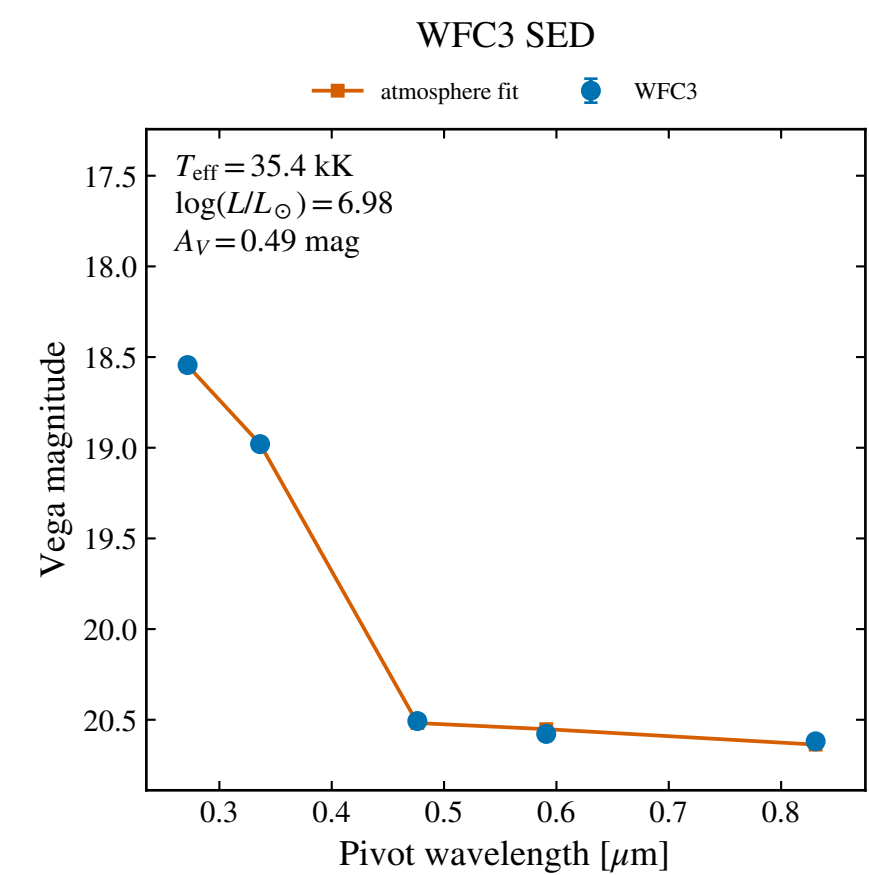
WFC3 F814W: 20.619 \pm 0.009
