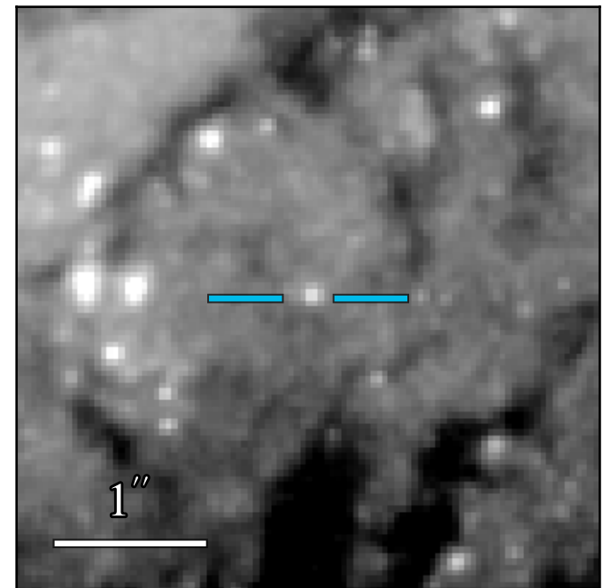
WFC3 F814W: 21.799 \pm 0.014
