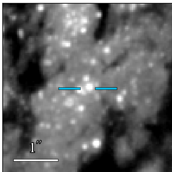
WFC3 F475W: 21.918 \pm 0.008
