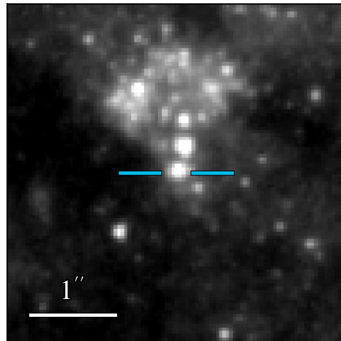
WFC3 F606W: 22.250 \pm 0.007
