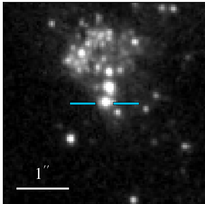
WFC3 F336W: 21.116 \pm 0.011
