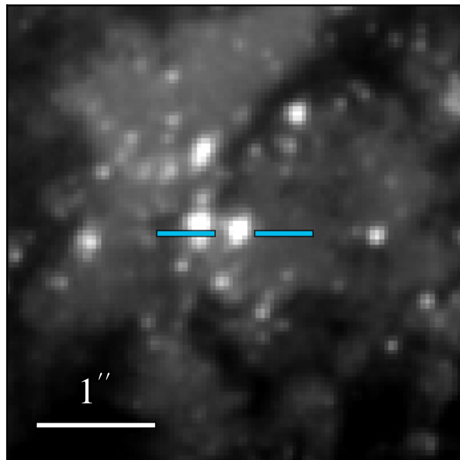
WFC3 F475W: 20.507 \pm 0.005
