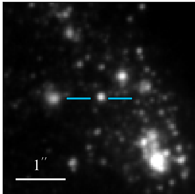
WFC3 F336W: 20.038 \pm 0.007
