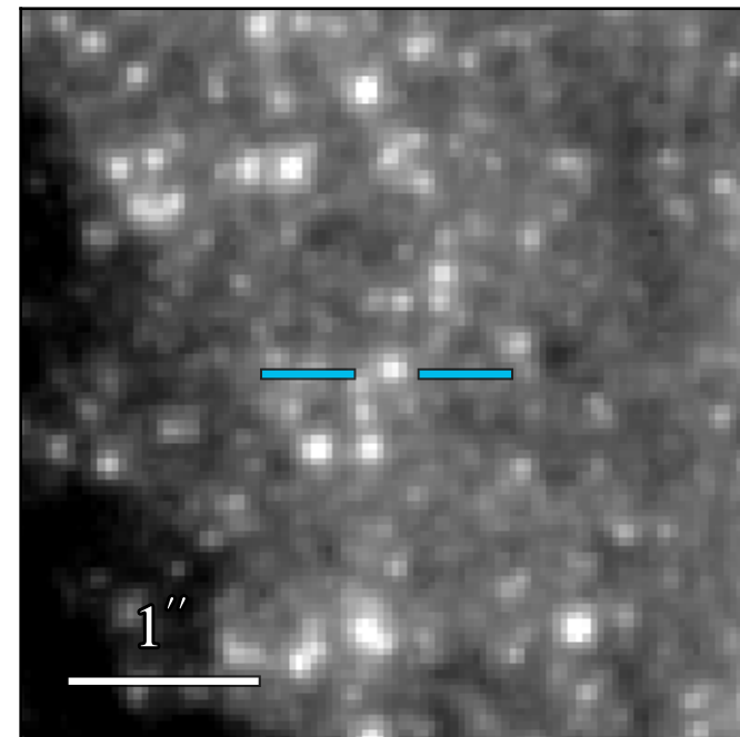
WFC3 F814W: 22.083 \pm 0.013
