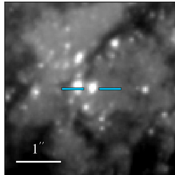
WFC3 F606W: 20.578 \pm 0.006
