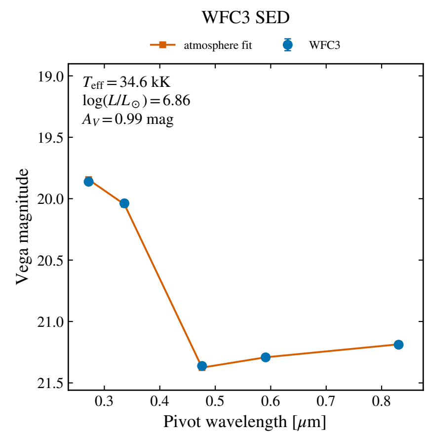
WFC3 F814W: 21.189 \pm 0.008
