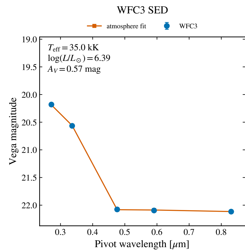
WFC3 F814W: 22.117 \pm 0.020
