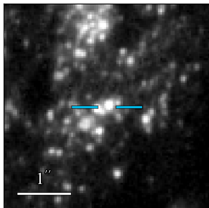
WFC3 F275W: 20.103 \pm 0.011
