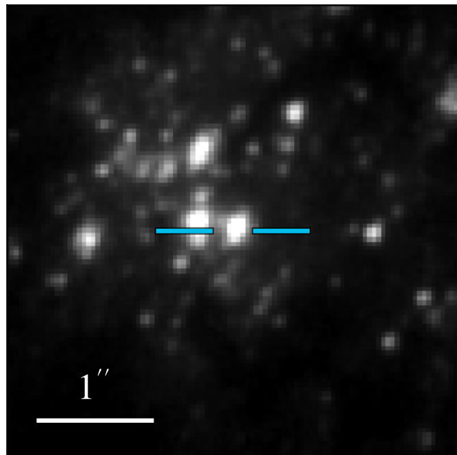
WFC3 F336W: 18.980 \pm 0.006
