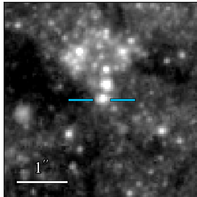
WFC3 F814W: 22.099 \pm 0.012
