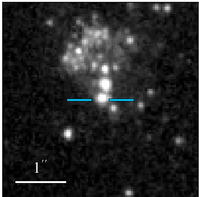
WFC3 F275W: 20.905 \pm 0.015
