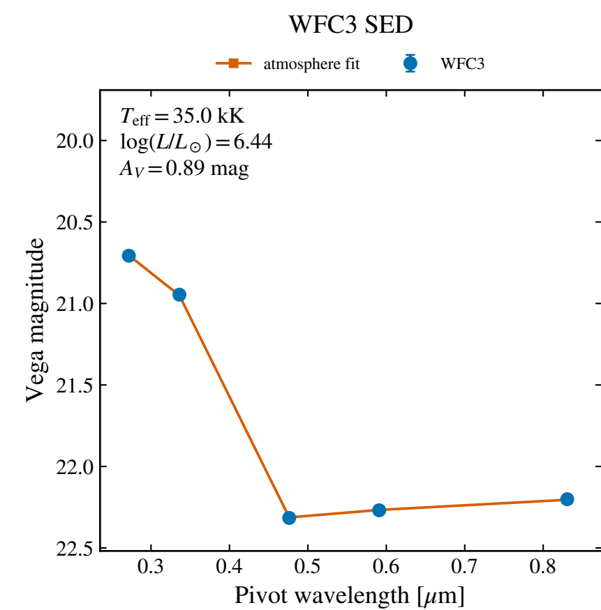
WFC3 F814W: 22.201 \pm 0.015
