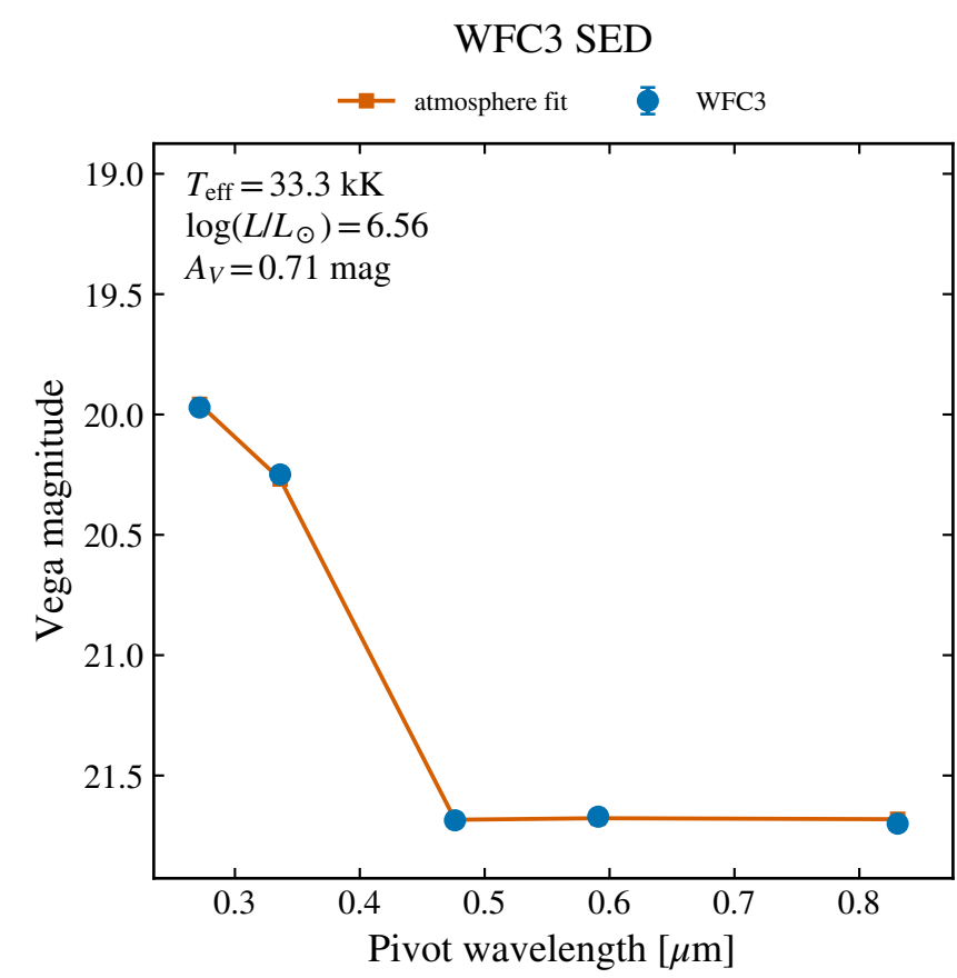
WFC3 F814W: 21.700 \pm 0.016
