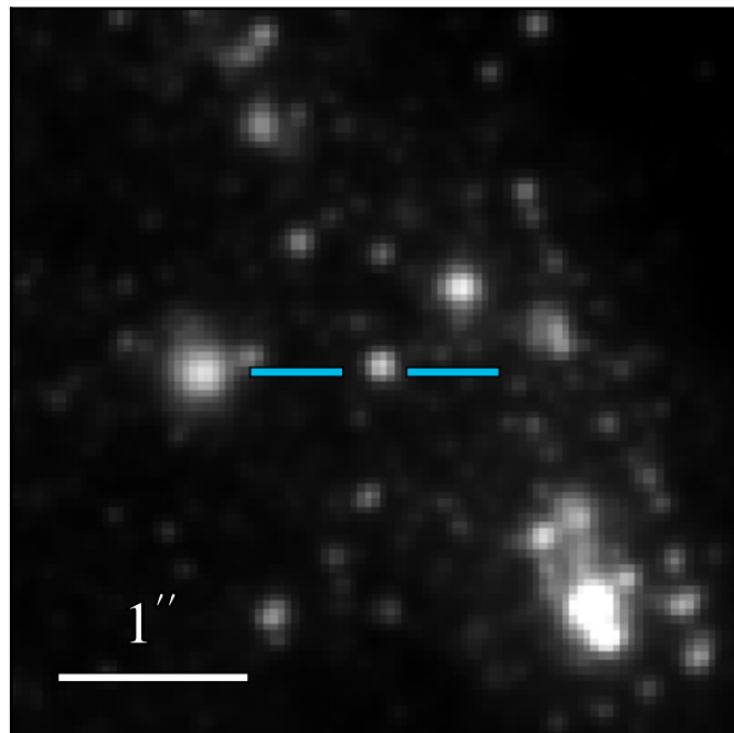
WFC3 F475W: 21.362 \pm 0.005
