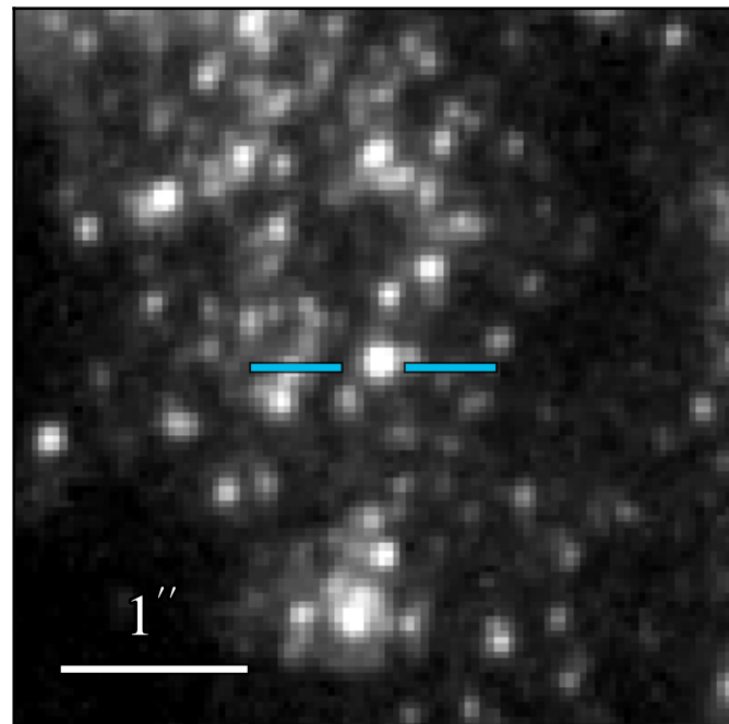
WFC3 F275W: 20.128 \pm 0.010
