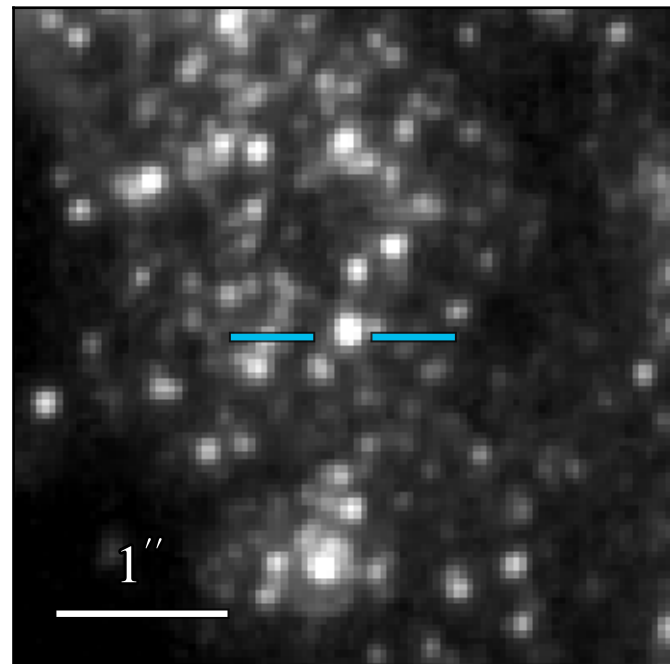
WFC3 F336W: 20.550 \pm 0.008
