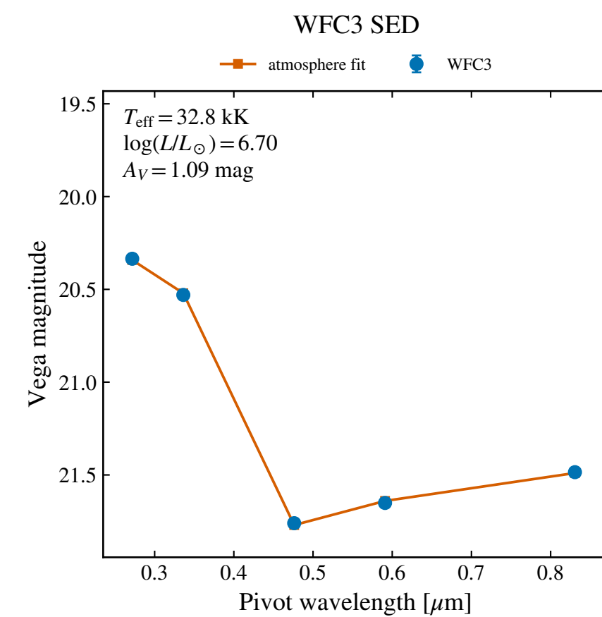
WFC3 F814W: 21.485 \pm 0.009
