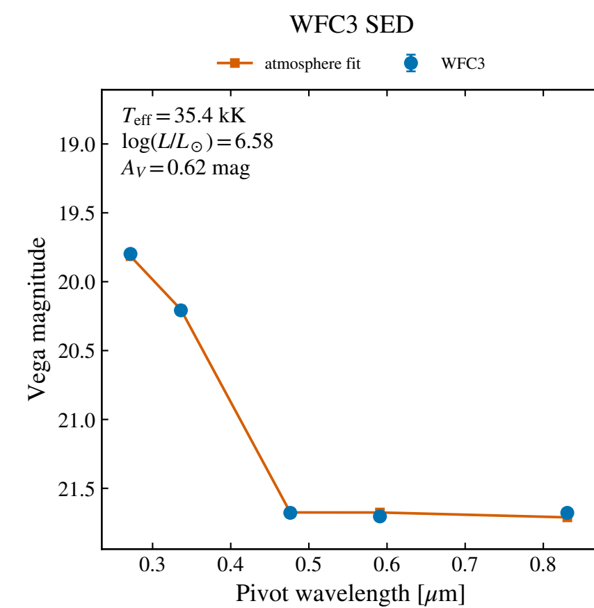
WFC3 F814W: 21.678 \pm 0.014
