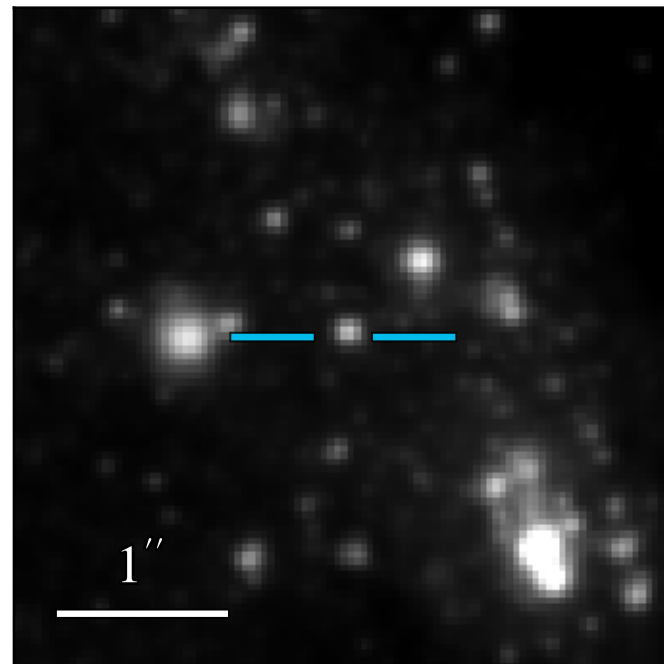
WFC3 F606W: 21.292 \pm 0.005
