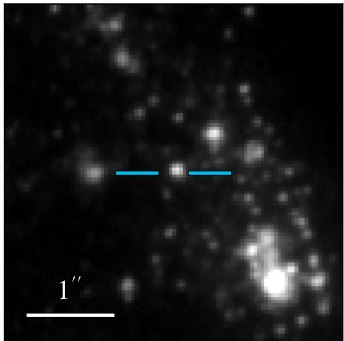
WFC3 F275W: 19.862 \pm 0.009
