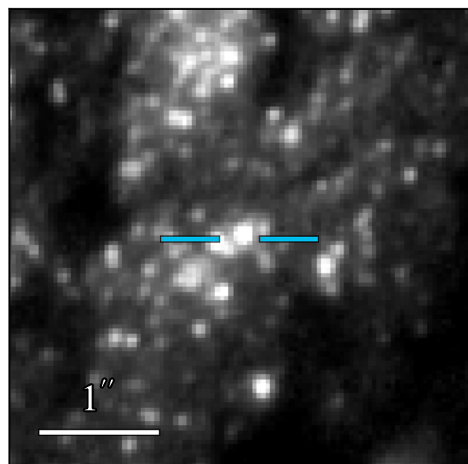
WFC3 F336W: 20.458 \pm 0.009
