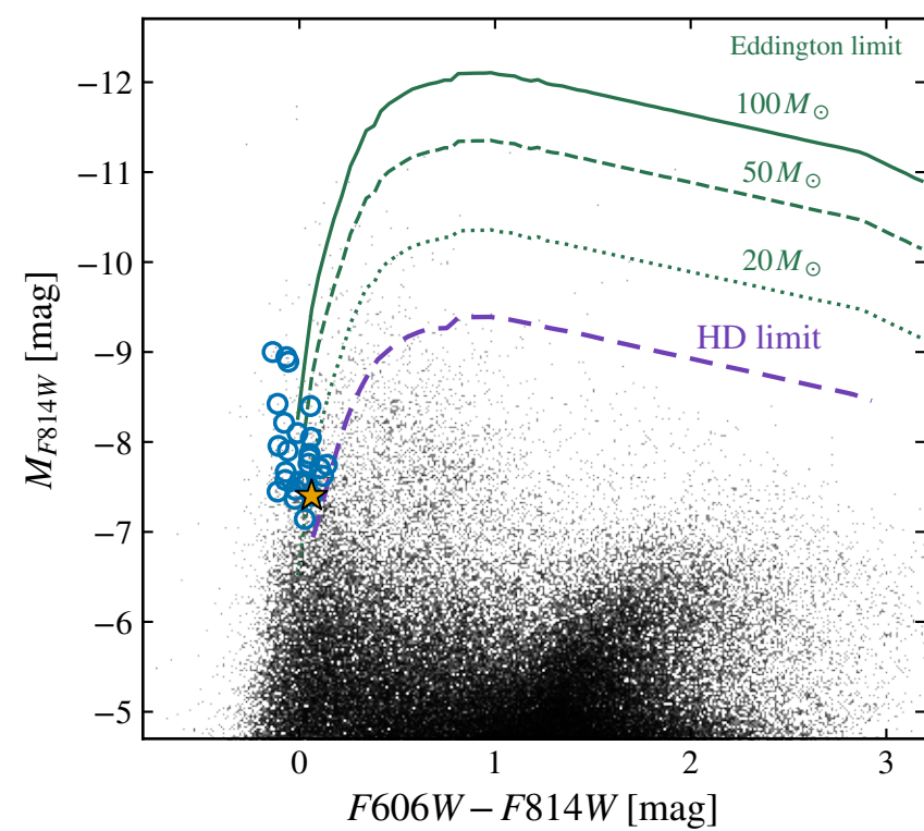
WFC3 F336W: 21.116 \pm 0.011
