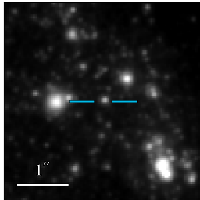
WFC3 F814W: 21.189 \pm 0.008
