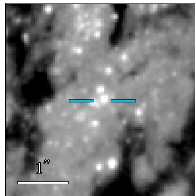
WFC3 F606W: 21.946 \pm 0.008
