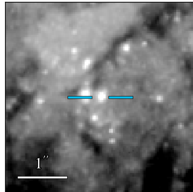
WFC3 F814W: 20.619 \pm 0.009
