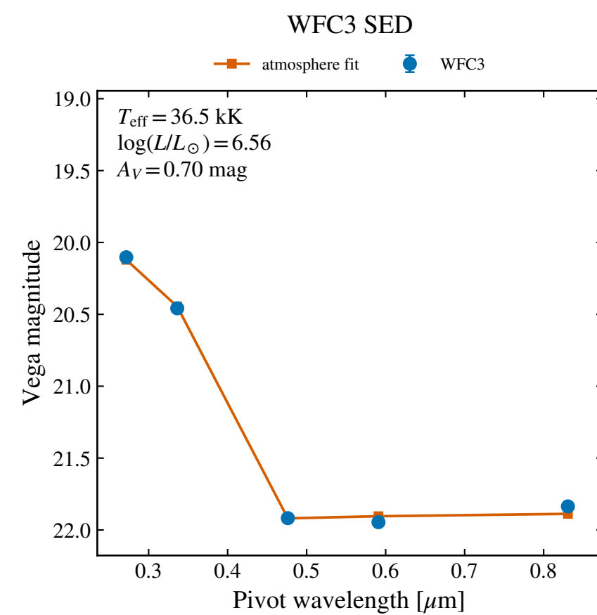
WFC3 F814W: 21.836 \pm 0.016
