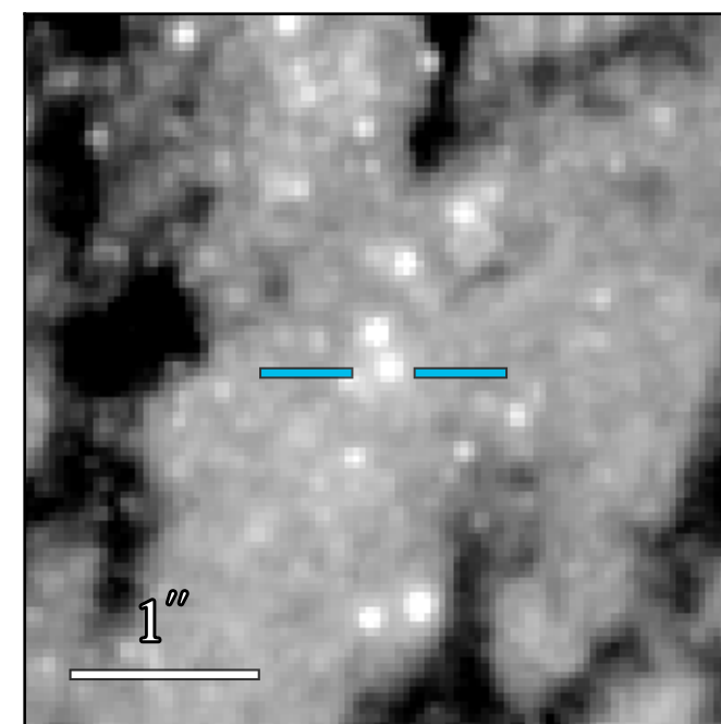
WFC3 F814W: 21.836 \pm 0.016
