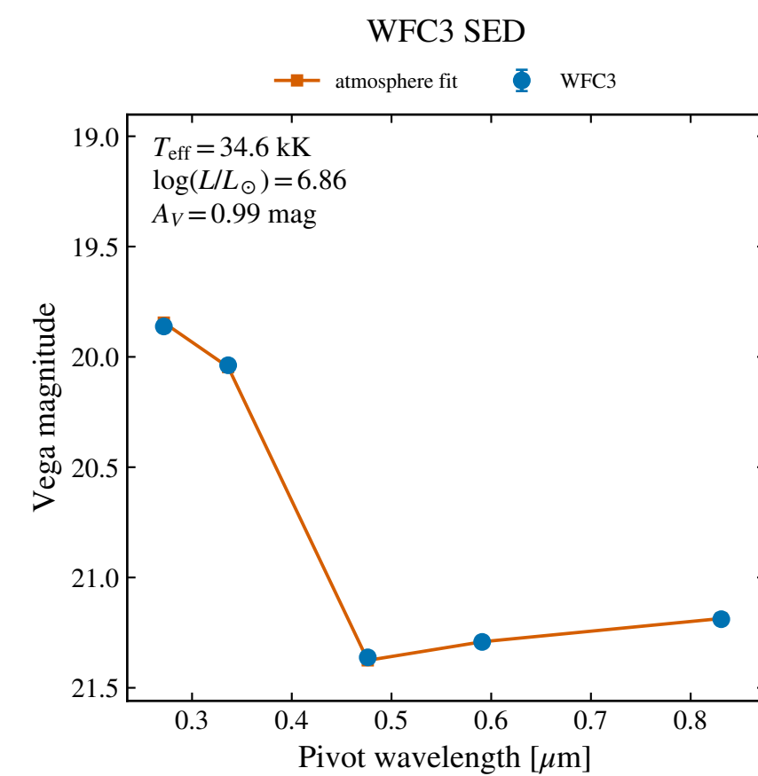
WFC3 F814W: 21.189 \pm 0.008
