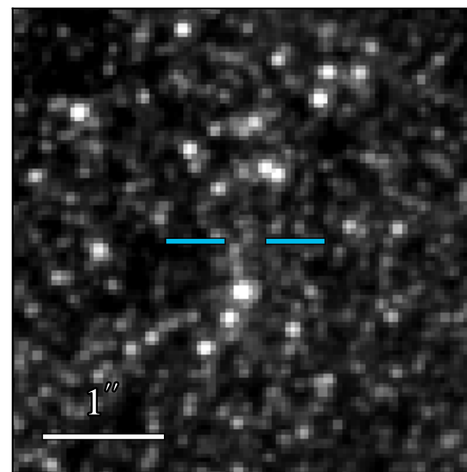
JWST/NIRCam F210M
