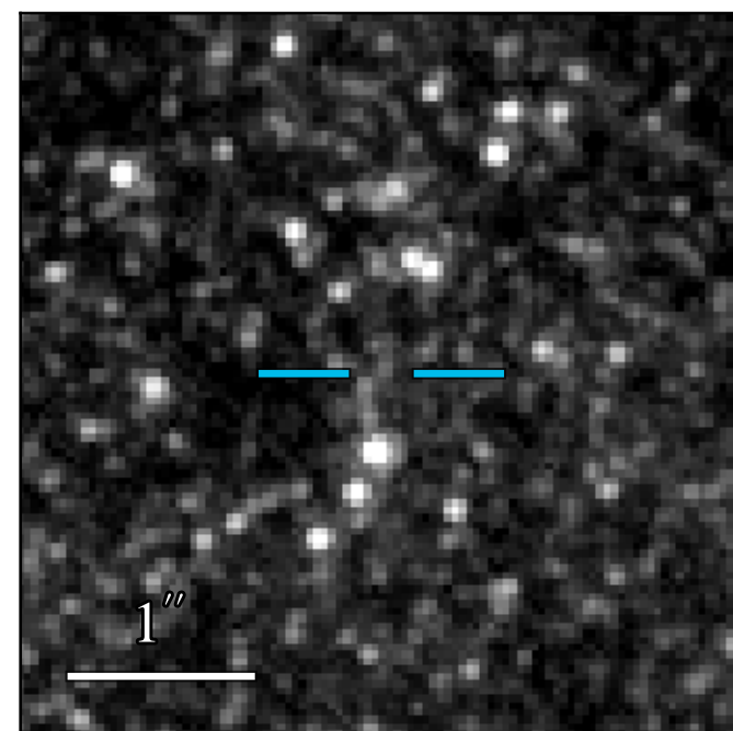
JWST/NIRCam F212N
