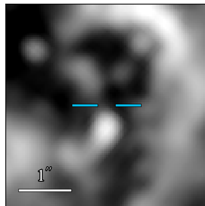
JWST/MIRI F1000W
