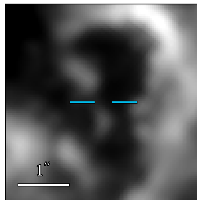
JWST/MIRI F770W
