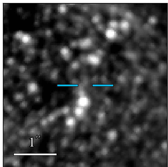
JWST/NIRCam F250M
