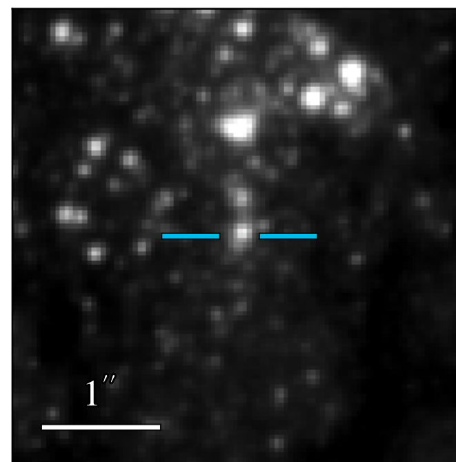
WFC3 F606W: 21.499 \pm 0.006
