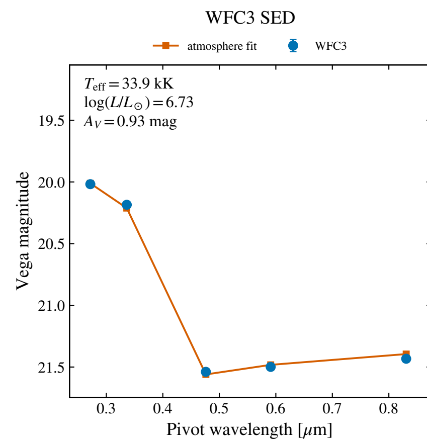
WFC3 F814W: 21.433 \pm 0.010
