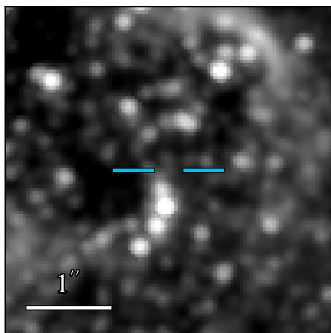
JWST/NIRCam F360M
