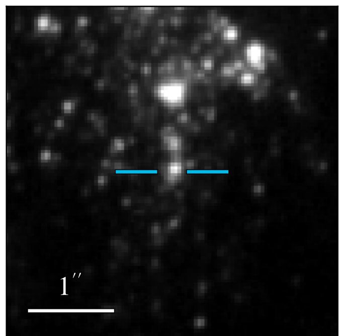
WFC3 F275W: 20.018 \pm 0.010
