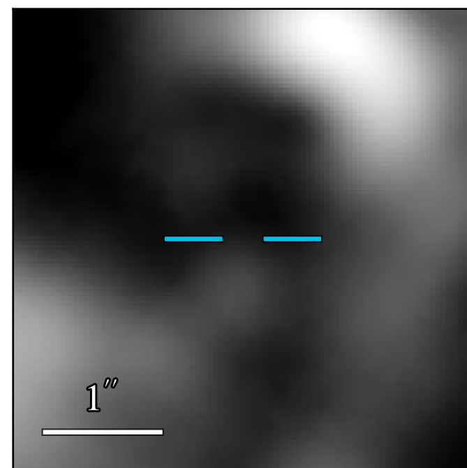
JWST/MIRI F2100W
