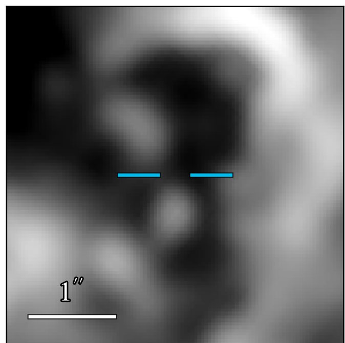
JWST/MIRI F1130W
