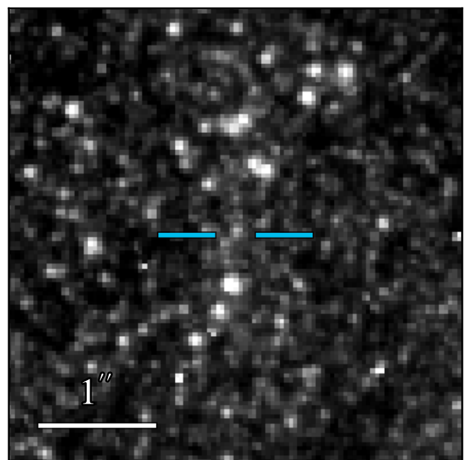
JWST/NIRCam F140M
