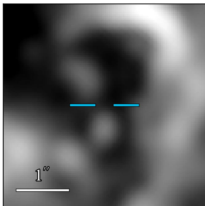
JWST/MIRI F1280W
