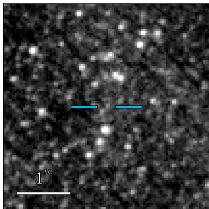
JWST/NIRCam F164N
