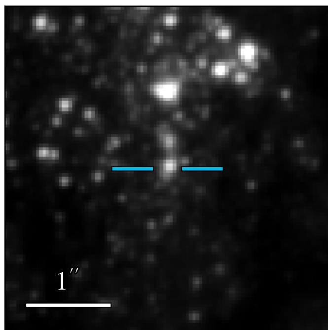
WFC3 F475W: 21.539 \pm 0.006
