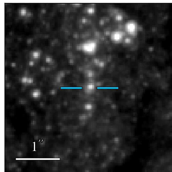
WFC3 F814W: 21.433 \pm 0.010
