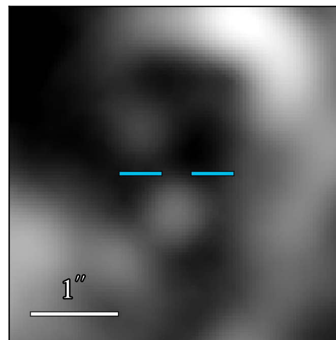
JWST/MIRI F1800W
