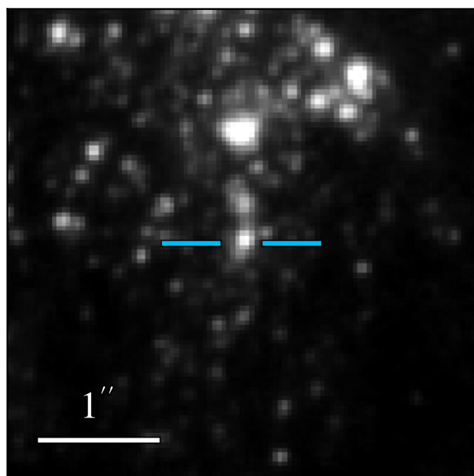
WFC3 F336W: 20.185 \pm 0.008
