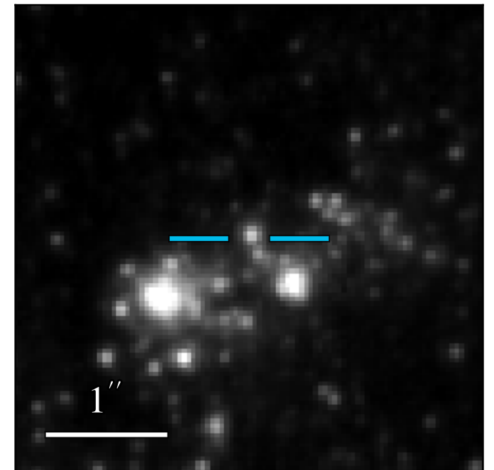
WFC3 F814W: 21.664 \pm 0.011
