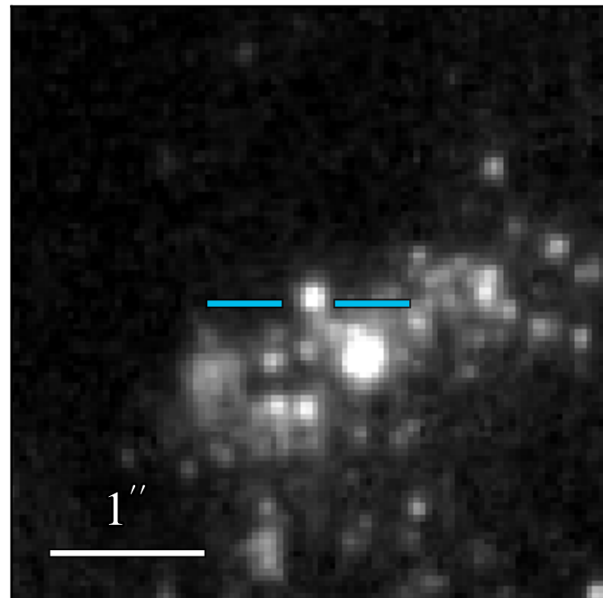
WFC3 F275W: 20.843 \pm 0.015
