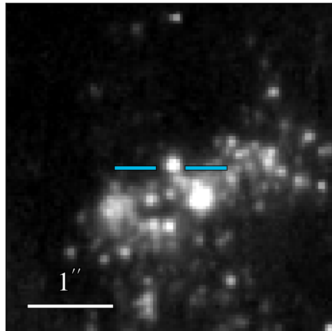
WFC3 F336W: 20.892 \pm 0.010
