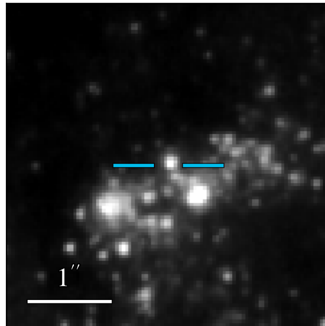
WFC3 F475W: 22.061 \pm 0.007
