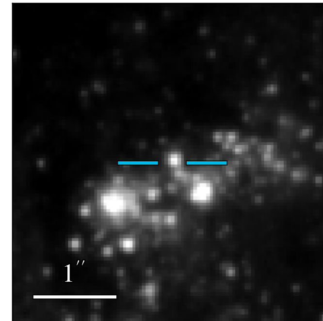
WFC3 F606W: 21.882 \pm 0.007
