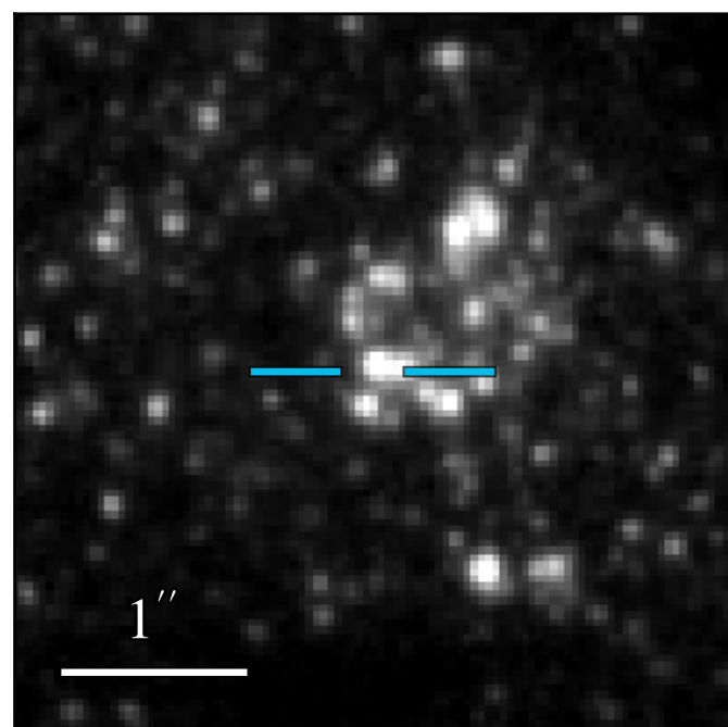
WFC3 F336W: 20.747 \pm 0.009
