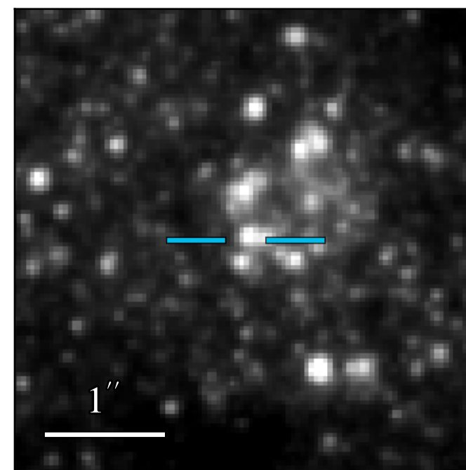
WFC3 F606W: 22.144 \pm 0.007
