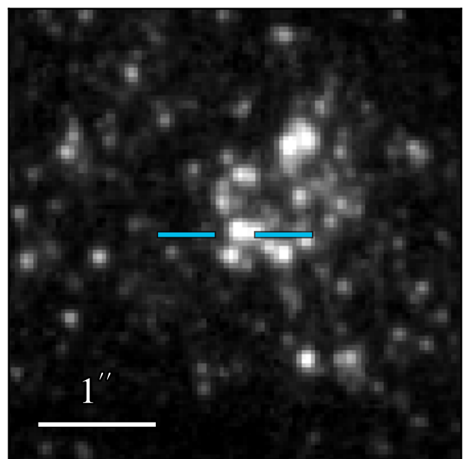
WFC3 F275W: 20.443 \pm 0.012
