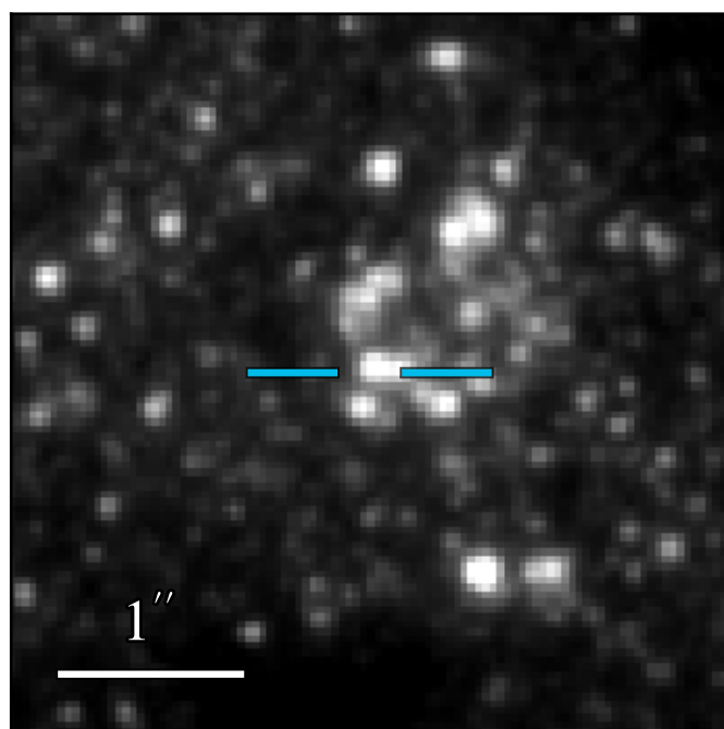
WFC3 F475W: 22.182 \pm 0.007
