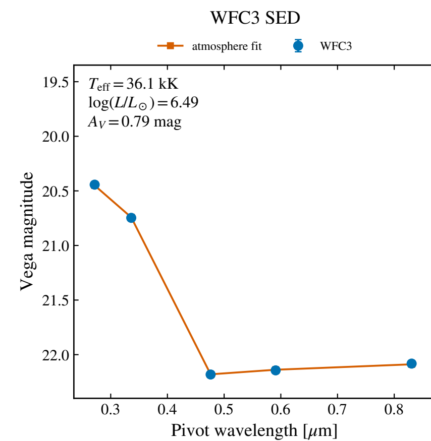
WFC3 F814W: 22.082 \pm 0.013
