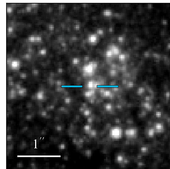
WFC3 F814W: 22.082 \pm 0.013
