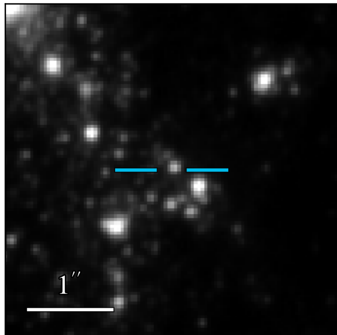
WFC3 F336W: 20.249 \pm 0.010
