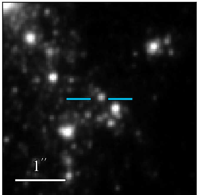
WFC3 F275W: 19.971 \pm 0.013
