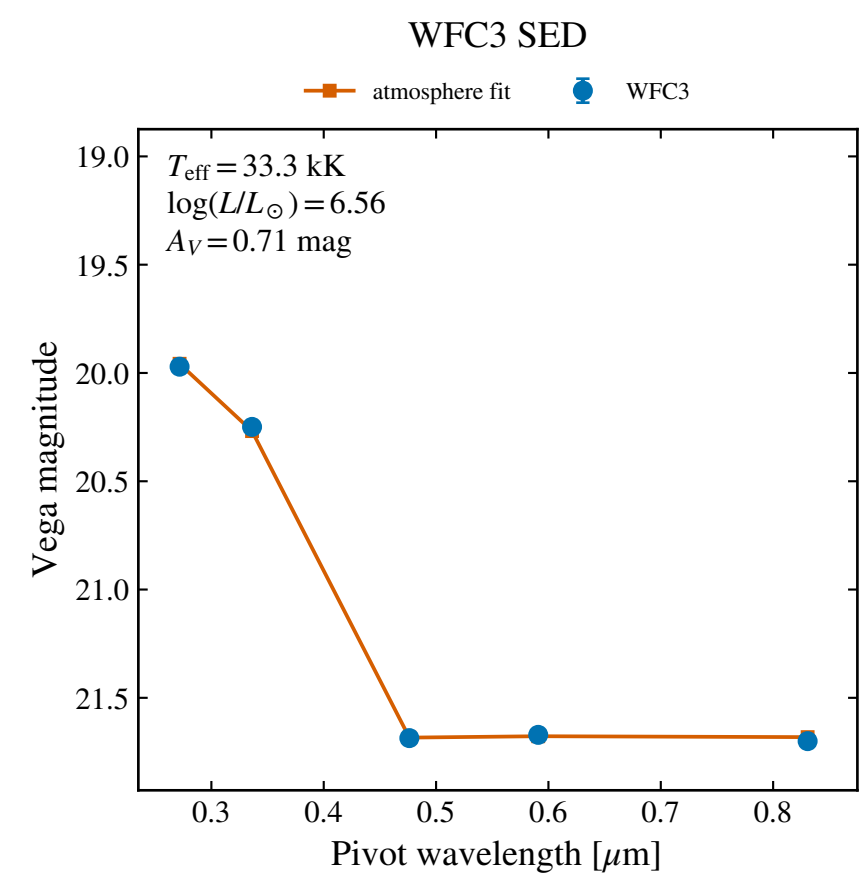
WFC3 F814W: 21.700 \pm 0.016
