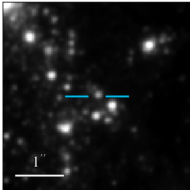
WFC3 F475W: 21.686 \pm 0.010
