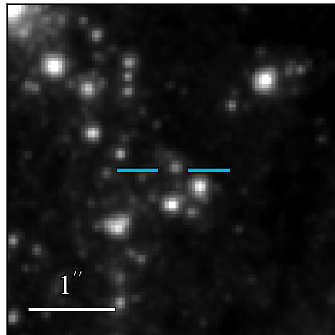
WFC3 F814W: 21.700 \pm 0.016
