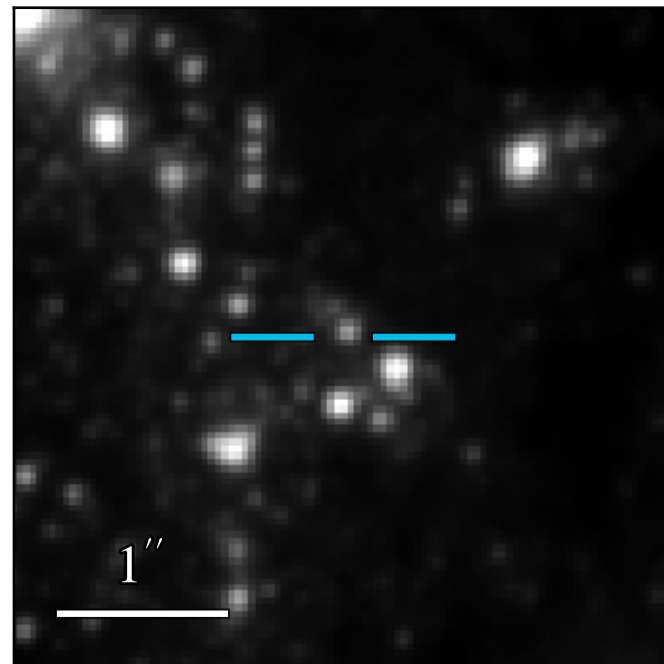
WFC3 F606W: 21.671 \pm 0.010
