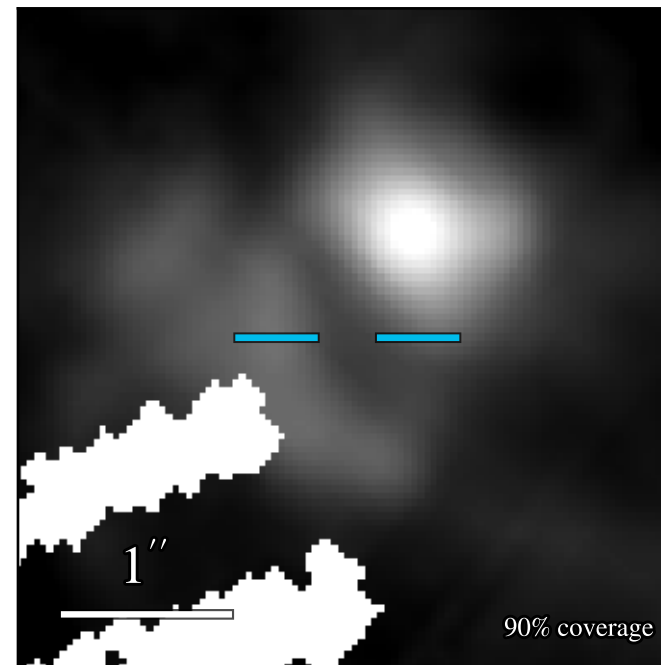
JWST/MIRI F1000W
