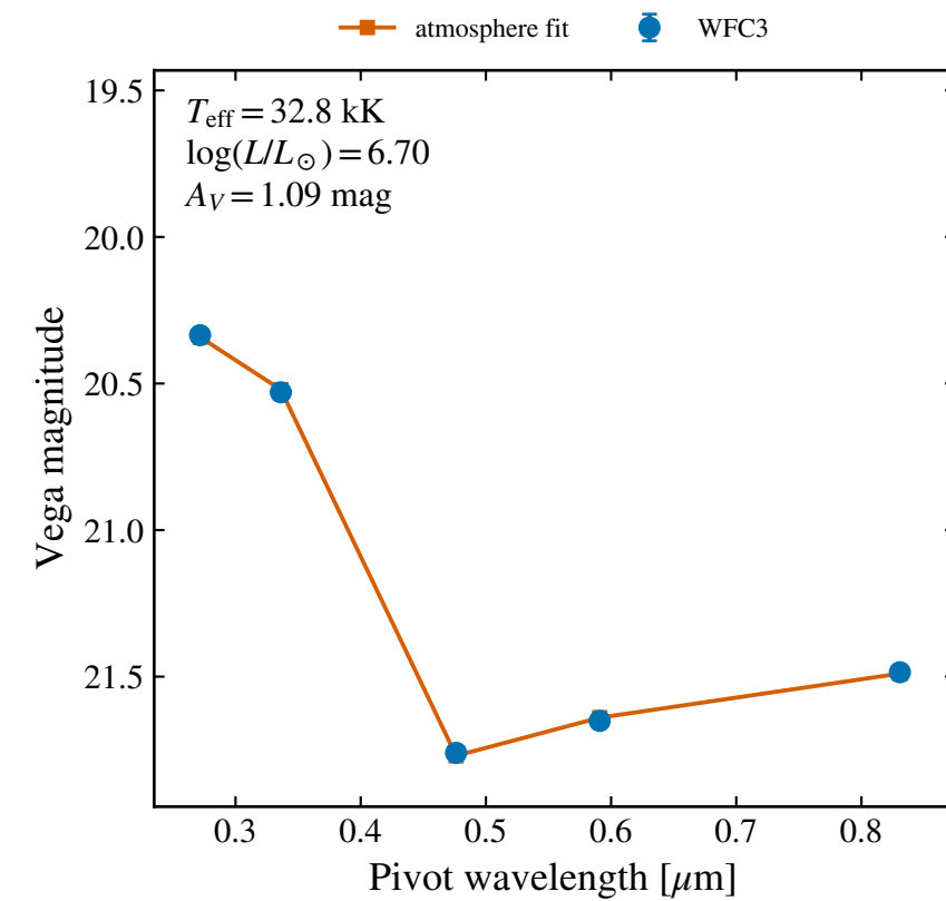
WFC3 SED
