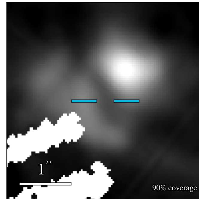
JWST/MIRI F1130W
