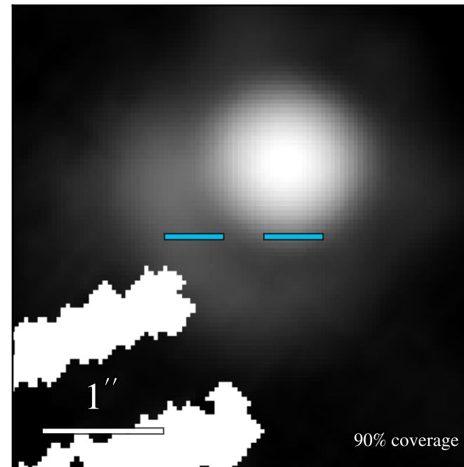
JWST/MIRI F2100W
