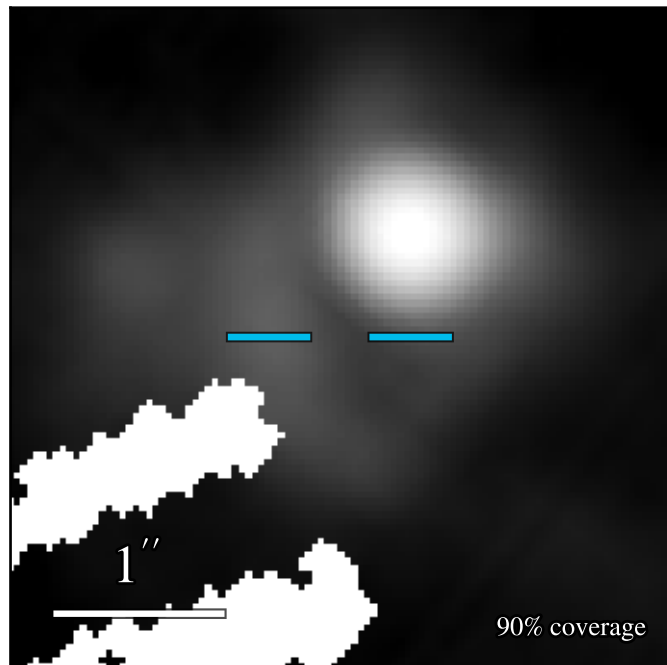
JWST/MIRI F1500W
