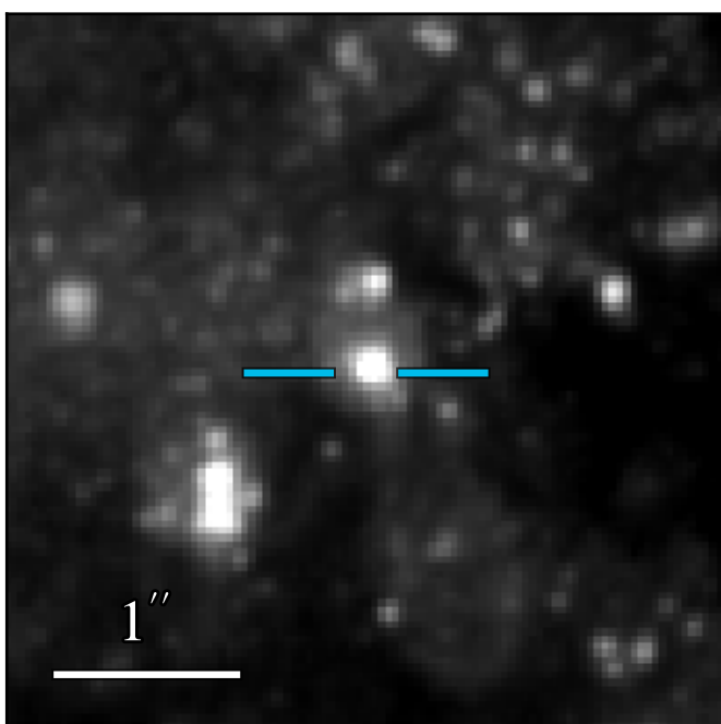
WFC3 F475W: 20.607 \pm 0.004
