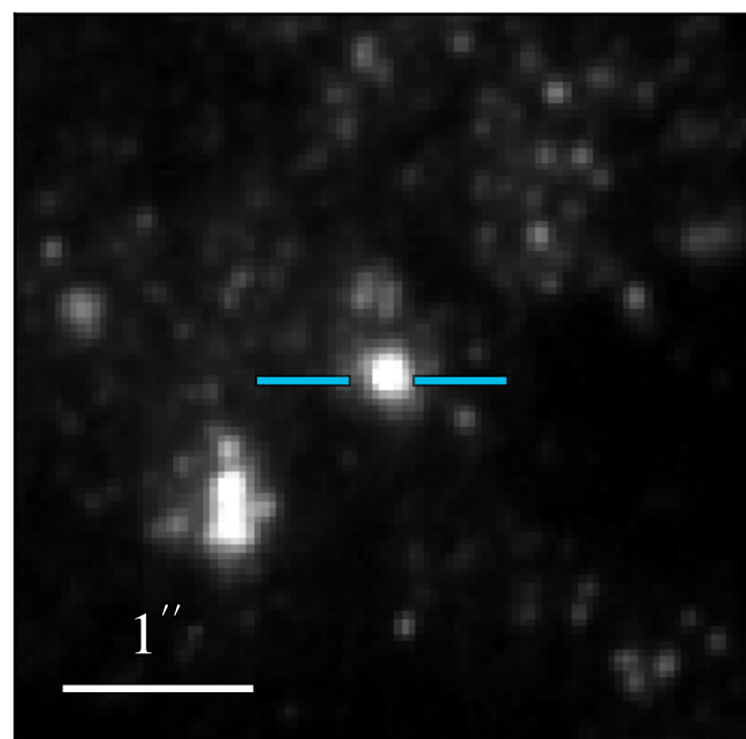
WFC3 F336W: 19.132 \pm 0.005
