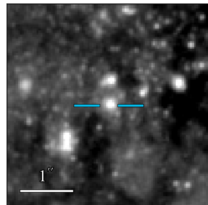
WFC3 F814W: 20.699 \pm 0.008
