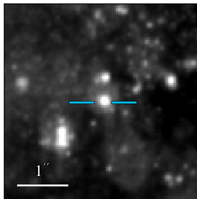
WFC3 F606W: 20.642 \pm 0.005
