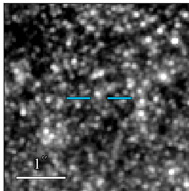
JWST/NIRCam F210M
