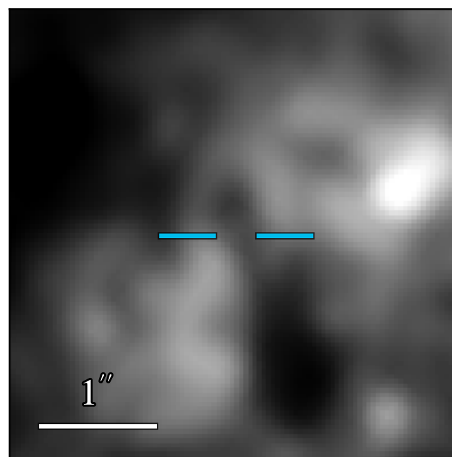
JWST/MIRI F770W
