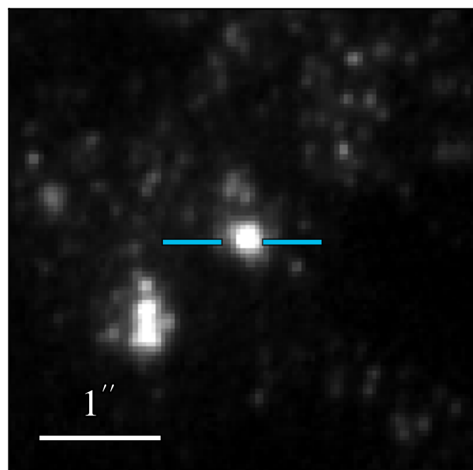
WFC3 F275W: 18.733 \pm 0.006
