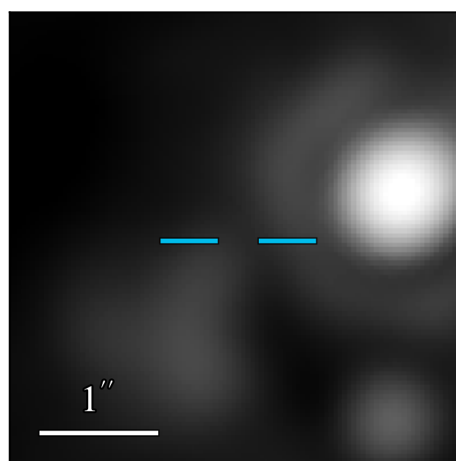
JWST/MIRI F1800W
