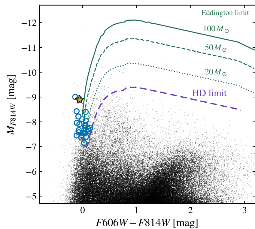
WFC3 F336W: 19.132 \pm 0.005
