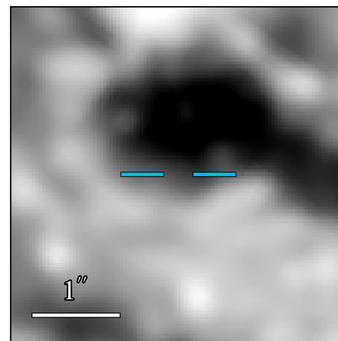
JWST/MIRI F770W
