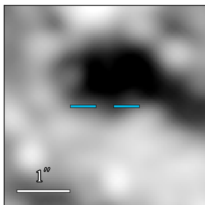
JWST/MIRI F1280W
