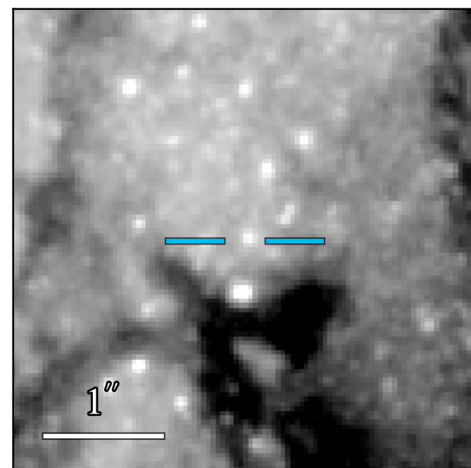
WFC3 F814W: 22.117 \pm 0.020
