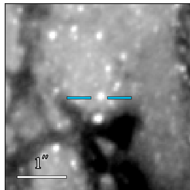
WFC3 F606W: 22.096 \pm 0.010
