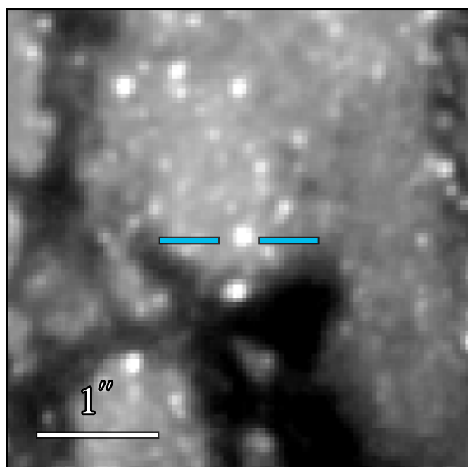
WFC3 F475W: 22.077 \pm 0.009
