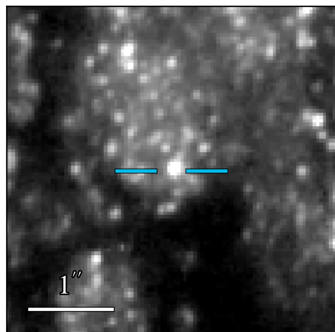
WFC3 F336W: 20.566 \pm 0.009
