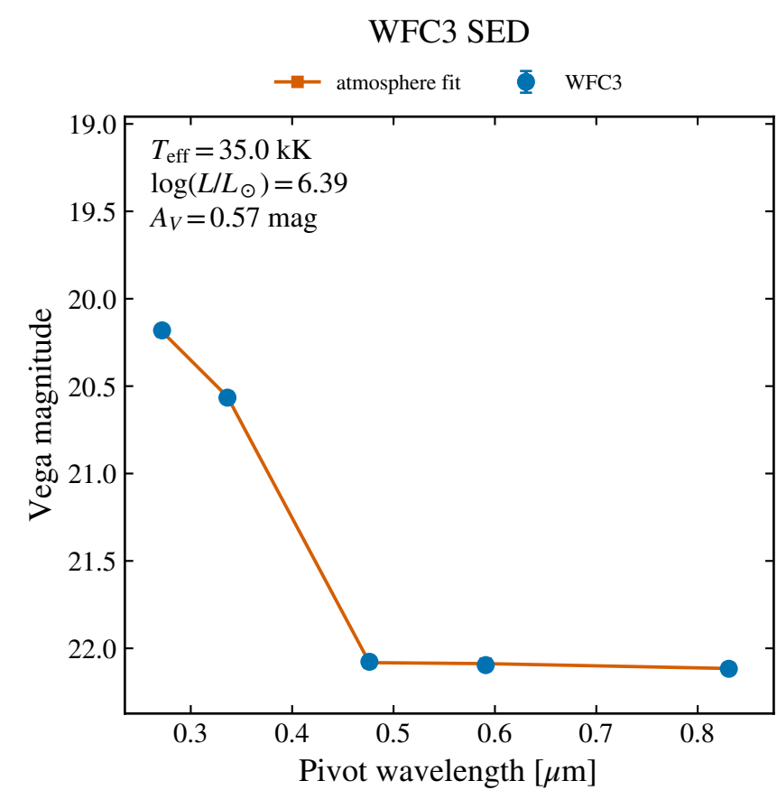
WFC3 F814W: 22.117 \pm 0.020
