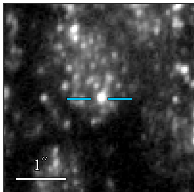
WFC3 F275W: 20.181 \pm 0.011
