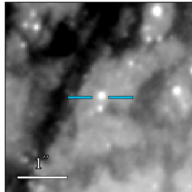
WFC3 F606W: 21.704 \pm 0.007
