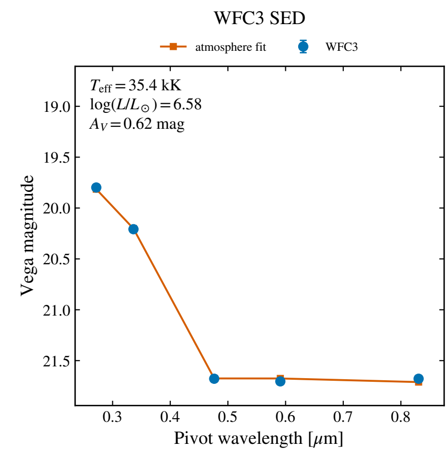
WFC3 F814W: 21.678 \pm 0.014
