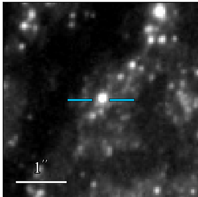
WFC3 F336W: 20.208 \pm 0.007
