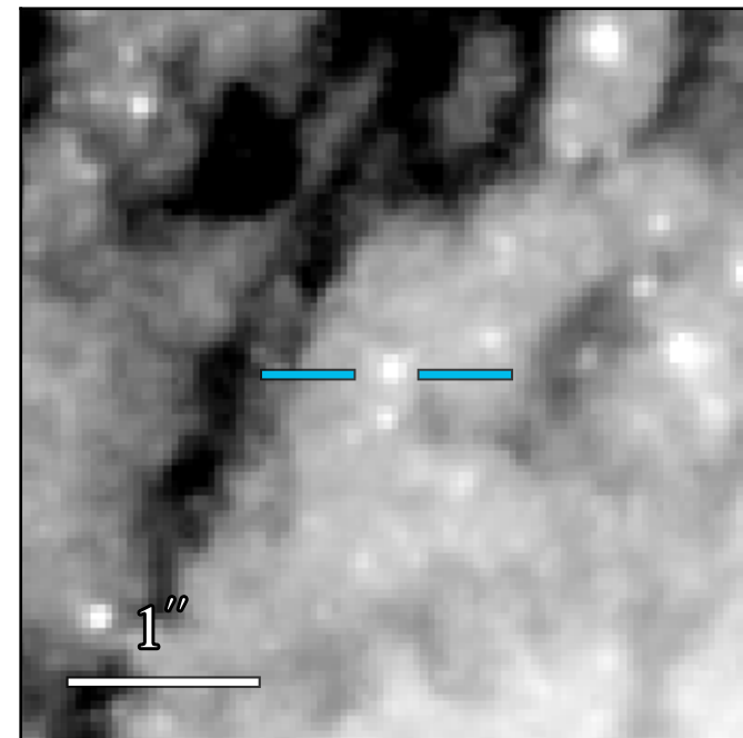
WFC3 F814W: 21.678 \pm 0.014
