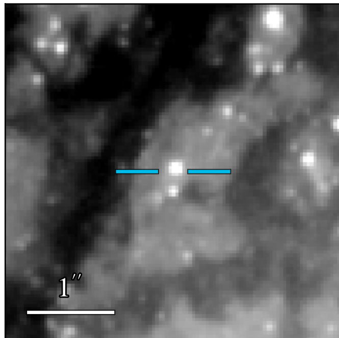
WFC3 F475W: 21.678 \pm 0.006
