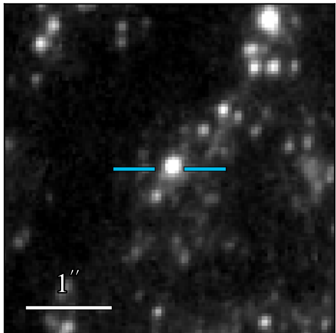
WFC3 F275W: 19.798 \pm 0.008
