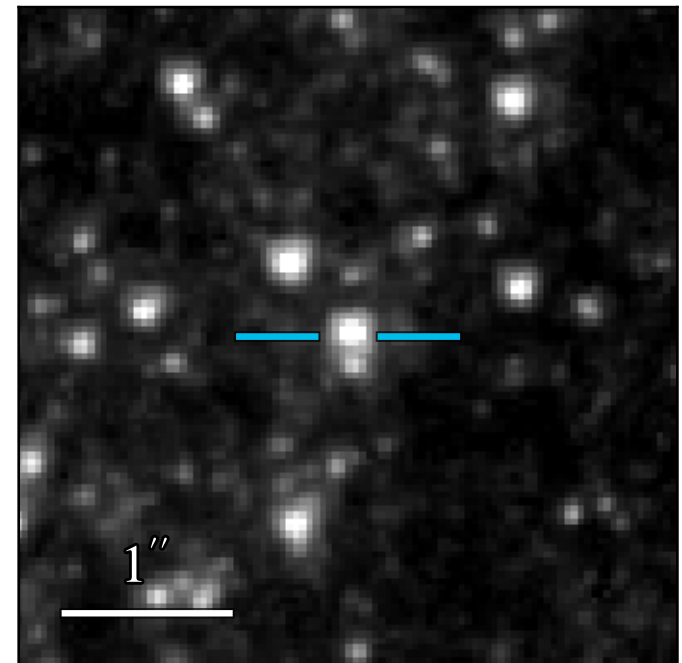
WFC3 F814W: 21.809 \pm 0.010
