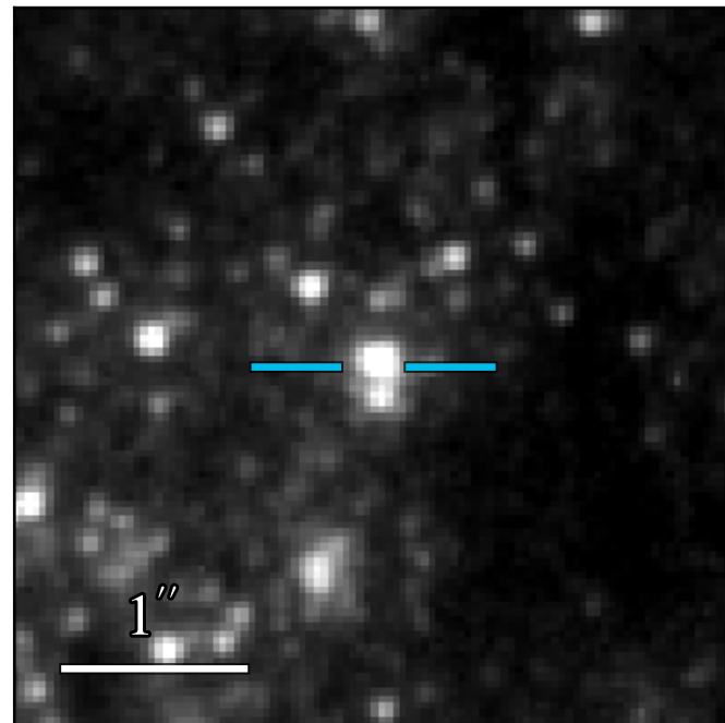
WFC3 F475W: 22.231 \pm 0.008
