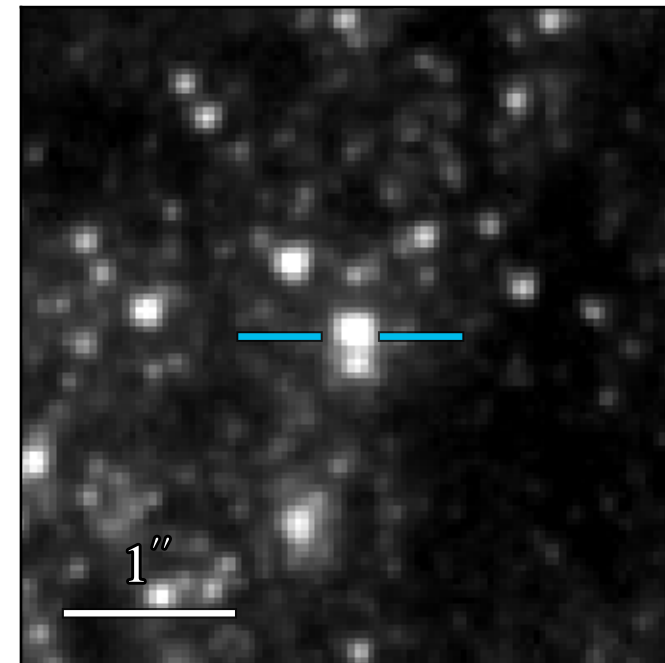
WFC3 F606W: 22.059 \pm 0.008
