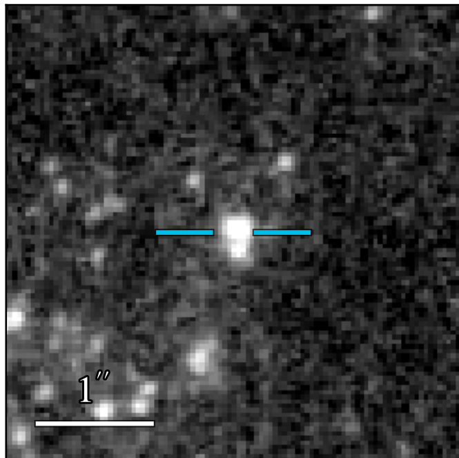
WFC3 F275W: 21.014 \pm 0.016
