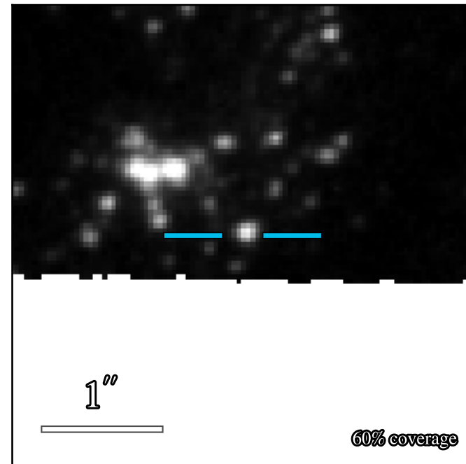
WFC3 F336W: 20.902 \pm 0.010
