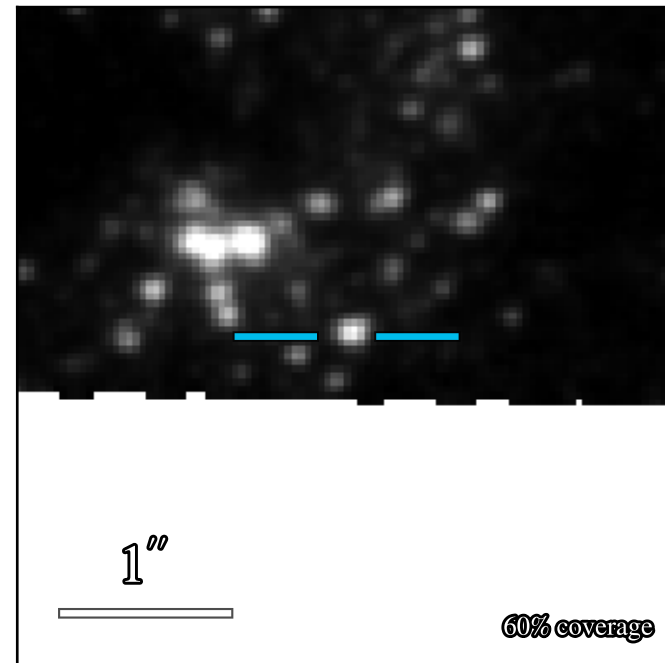
WFC3 F475W: 22.250 \pm 0.008
