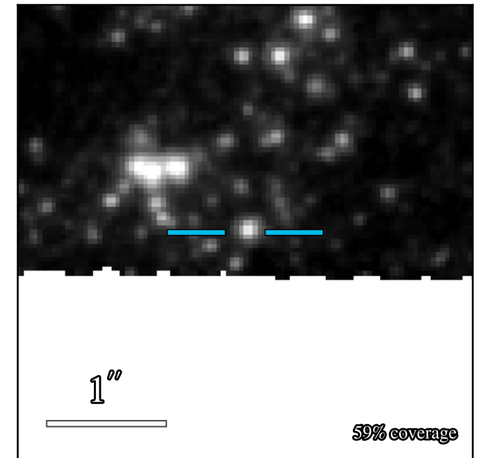
WFC3 F814W: 22.054 \pm 0.011
