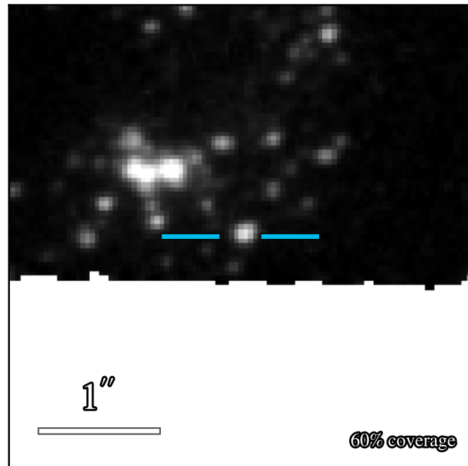
WFC3 F275W: 20.677 \pm 0.015
