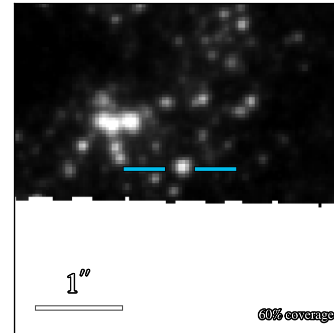
WFC3 F606W: 22.142 \pm 0.007
