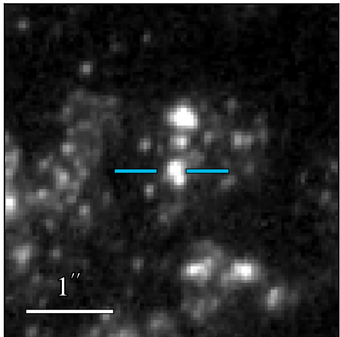
WFC3 F275W: 20.729 \pm 0.014
