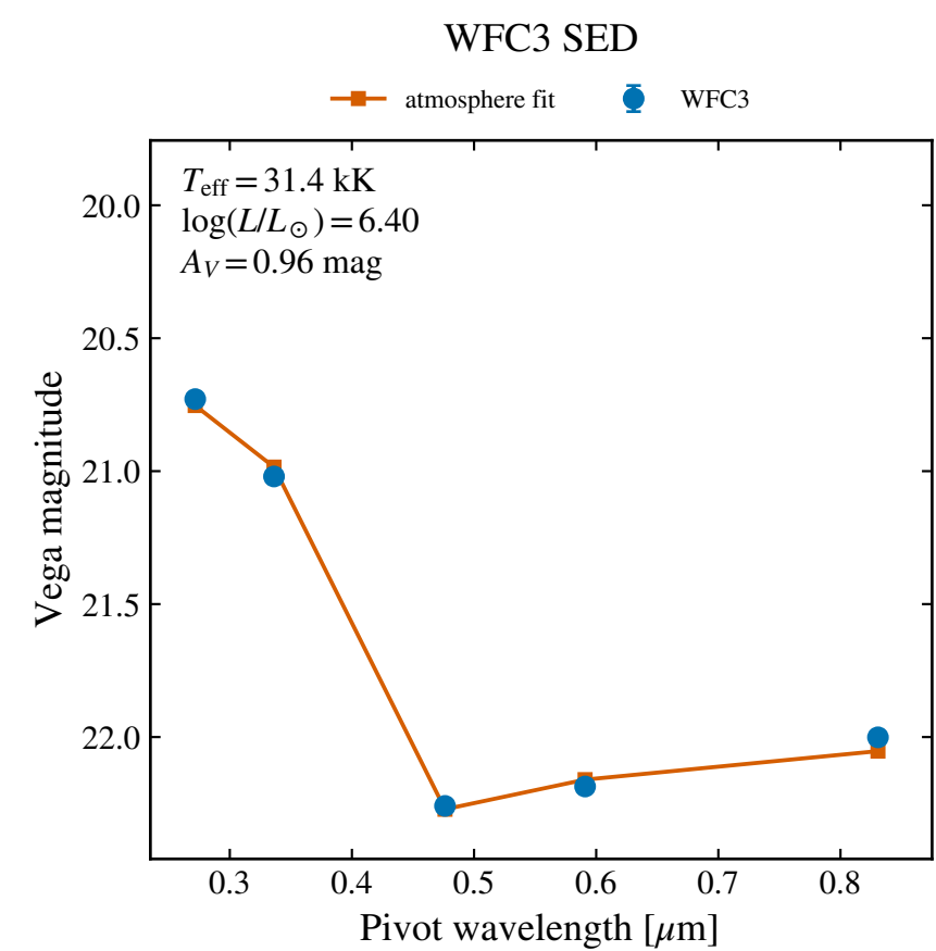
WFC3 F814W: 22.001 \pm 0.018
