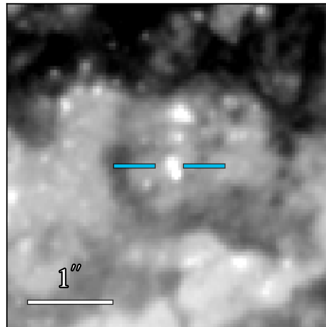
WFC3 F606W: 22.186 \pm 0.010
