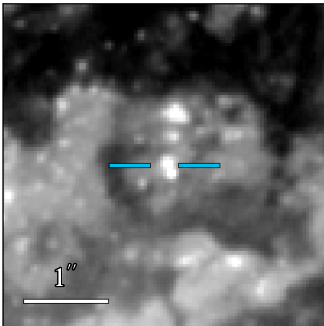
WFC3 F475W: 22.259 \pm 0.009
