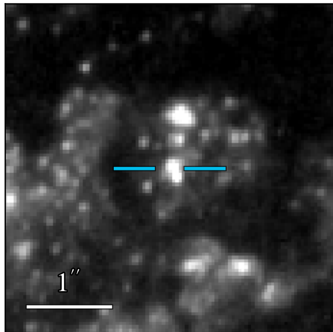
WFC3 F336W: 21.020 \pm 0.011
