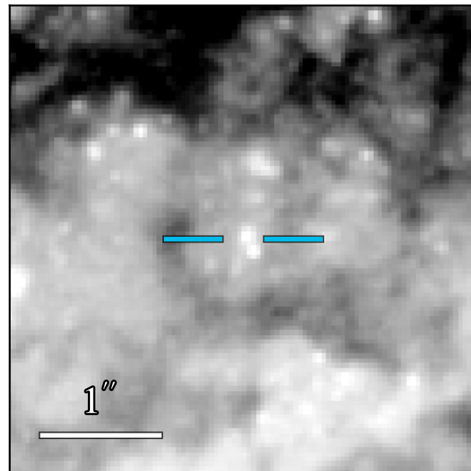
WFC3 F814W: 22.001 \pm 0.018
