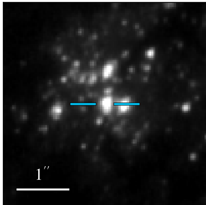
WFC3 F336W: 18.896 \pm 0.008
