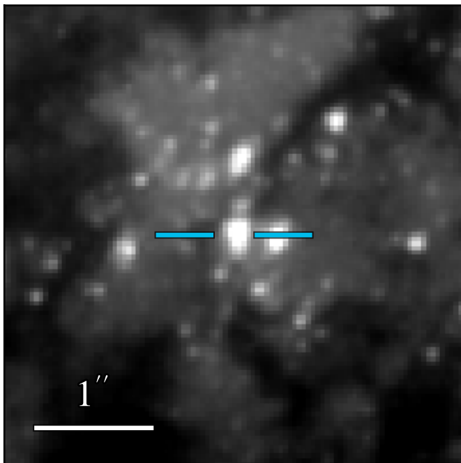
WFC3 F475W: 20.440 \pm 0.008
