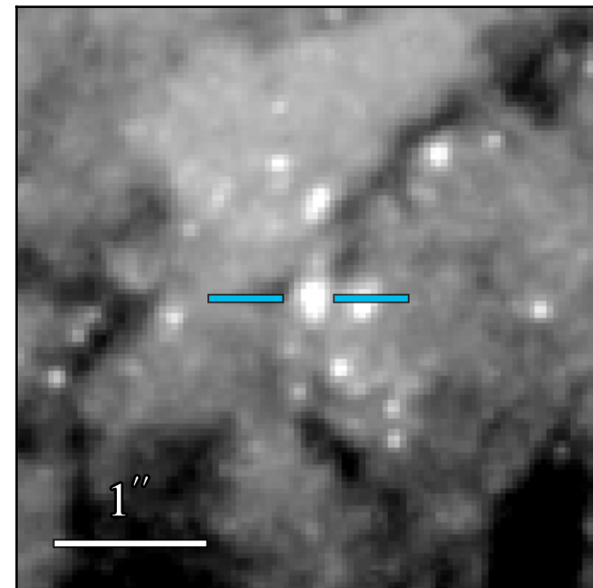
WFC3 F814W: 20.596 \pm 0.012
