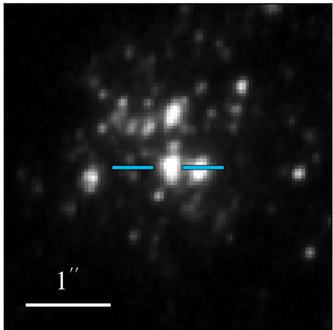
WFC3 F275W: 18.431 \pm 0.009
