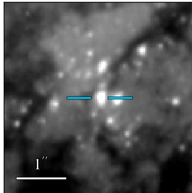
WFC3 F606W: 20.524 \pm 0.010
