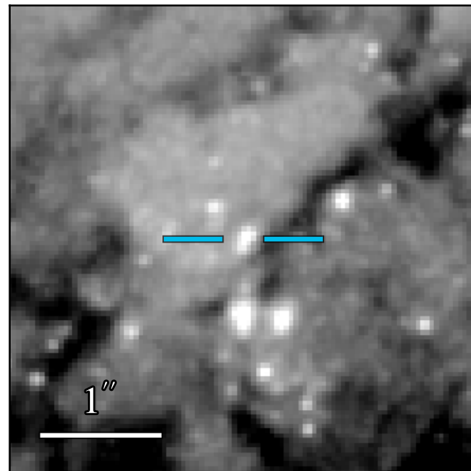
WFC3 F814W: 21.241 \pm 0.015
