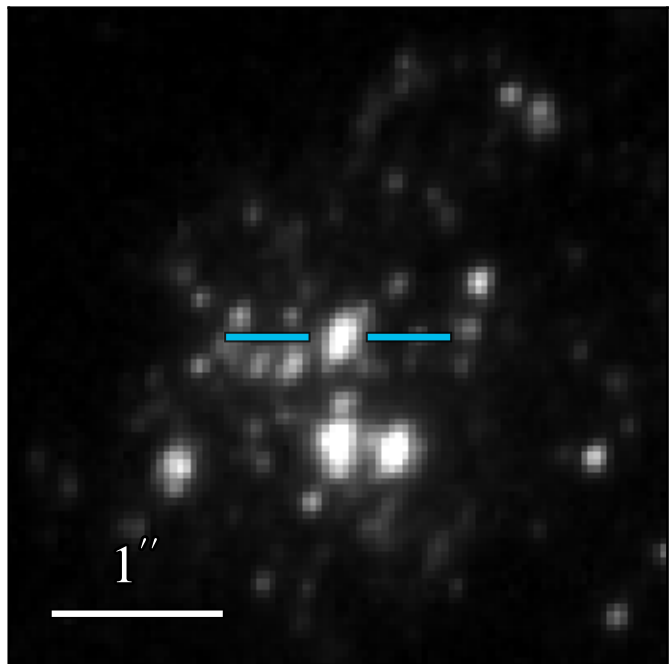
WFC3 F275W: 19.318 \pm 0.009
