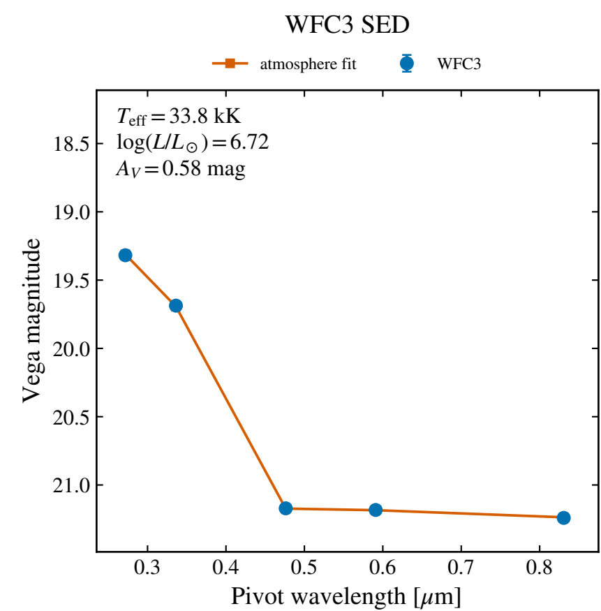
WFC3 F814W: 21.241 \pm 0.015
