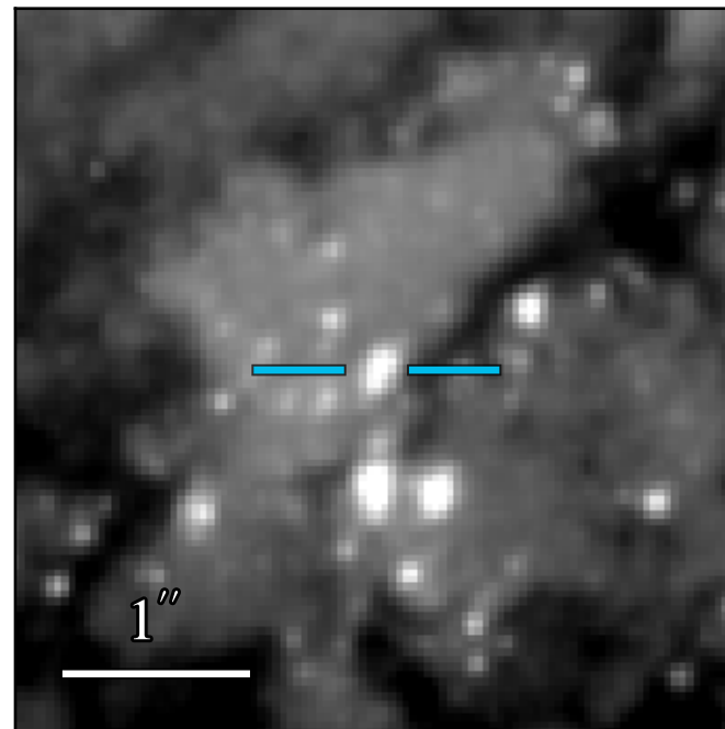
WFC3 F606W: 21.183 \pm 0.008
