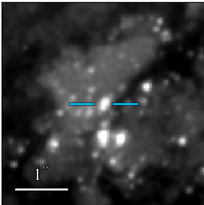
WFC3 F475W: 21.171 \pm 0.006
