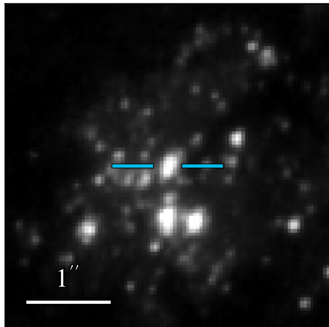
WFC3 F336W: 19.687 \pm 0.008
