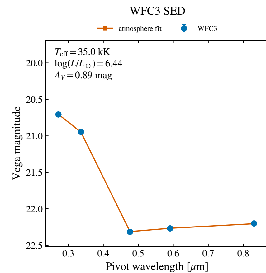
WFC3 F814W: 22.201 \pm 0.015
