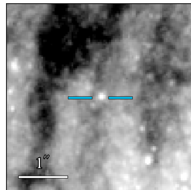
WFC3 F814W: 22.201 \pm 0.015
