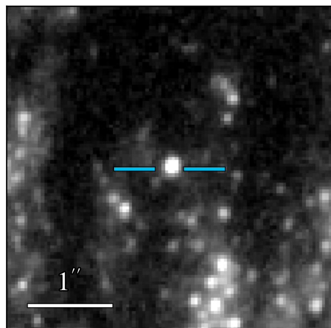
WFC3 F336W: 20.946 \pm 0.009
