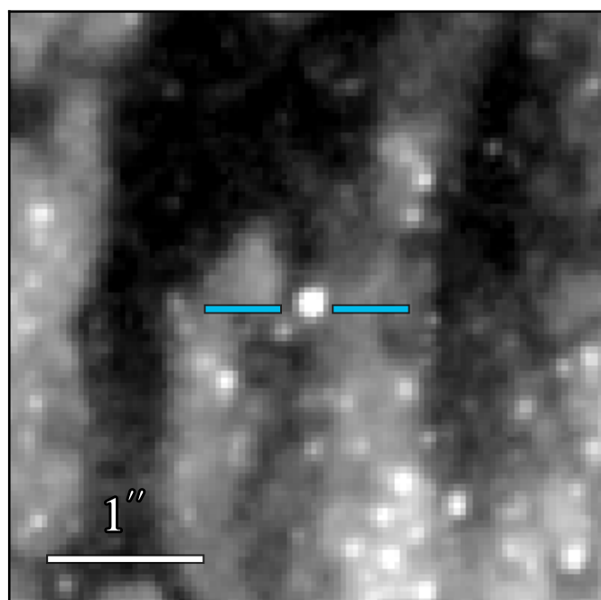
WFC3 F475W: 22.316 \pm 0.007
