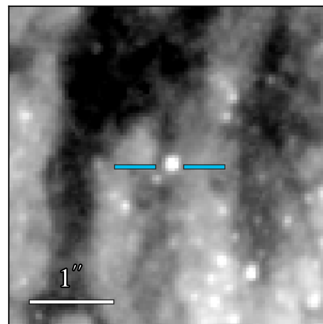
WFC3 F606W: 22.269 \pm 0.007
