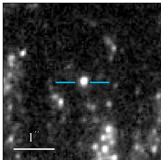
WFC3 F275W: 20.707 \pm 0.013
