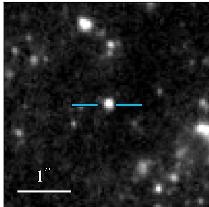
WFC3 F275W: 21.129 \pm 0.016
