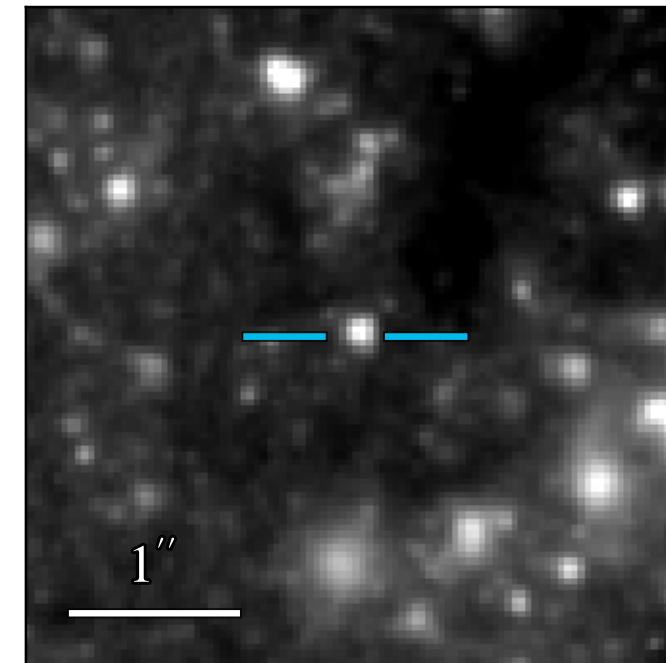
WFC3 F606W: 22.490 \pm 0.007
