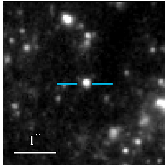
WFC3 F336W: 21.285 \pm 0.011
