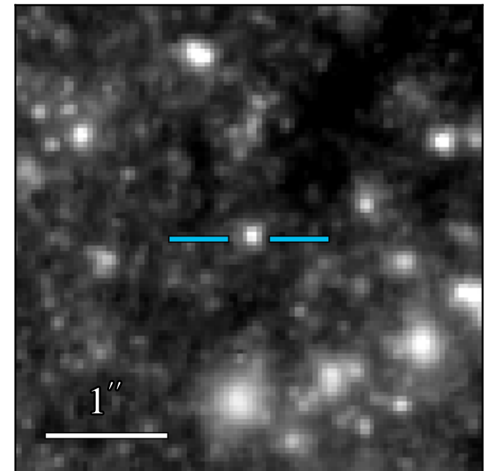
WFC3 F814W: 22.362 \pm 0.014
