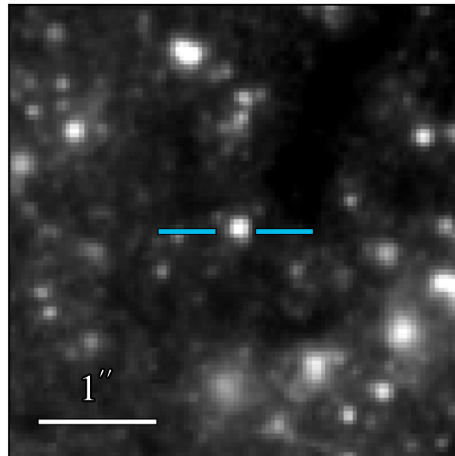
WFC3 F475W: 22.616 \pm 0.008
