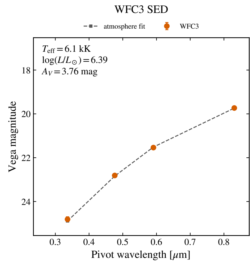
WFC3 F606W 21.539 ± 0.005
