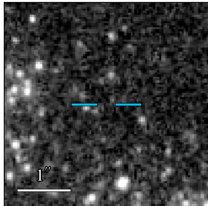
WFC3 F275W
