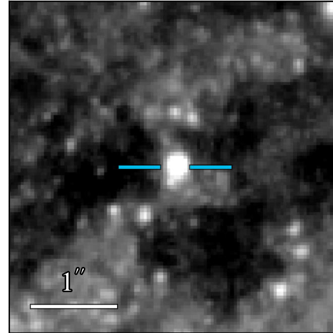
WFC3 F606W 21.539 ± 0.005
