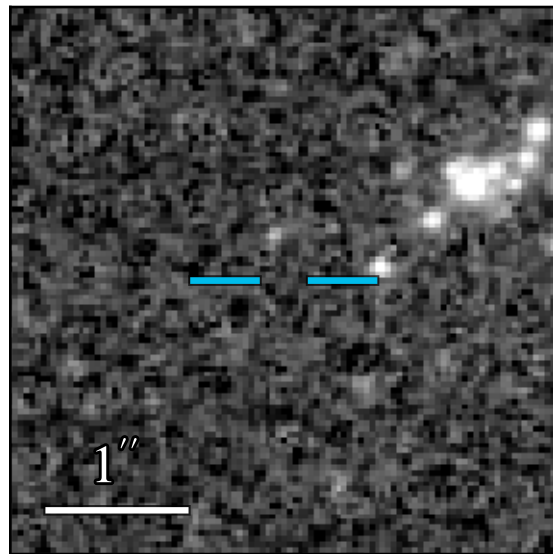
WFC3 F275W
