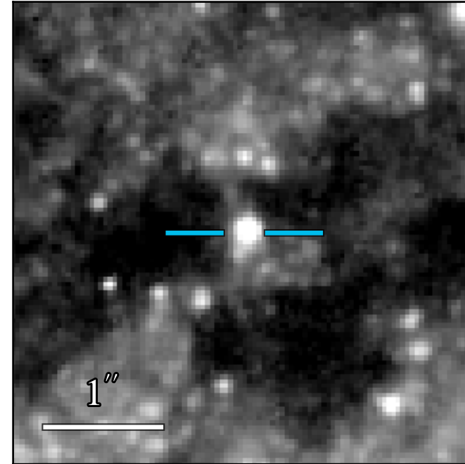
WFC3 F475W 22.811 ± 0.010
