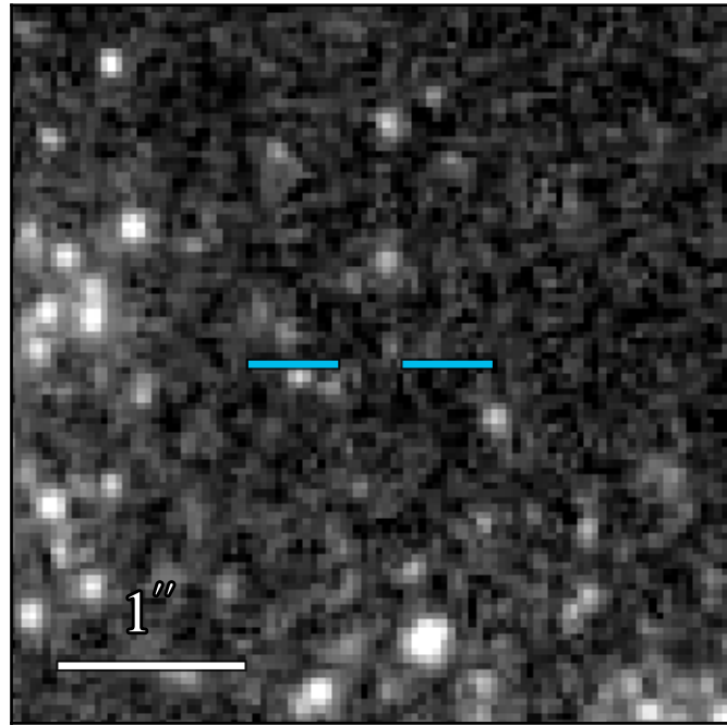
WFC3 F275W
