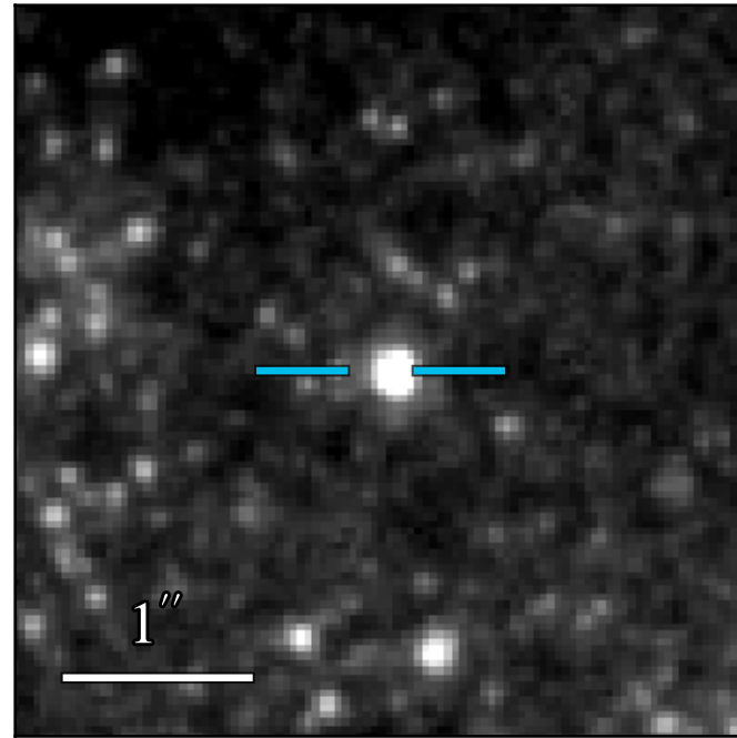
WFC3 F606W
