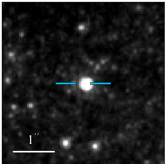
WFC3 F814W
