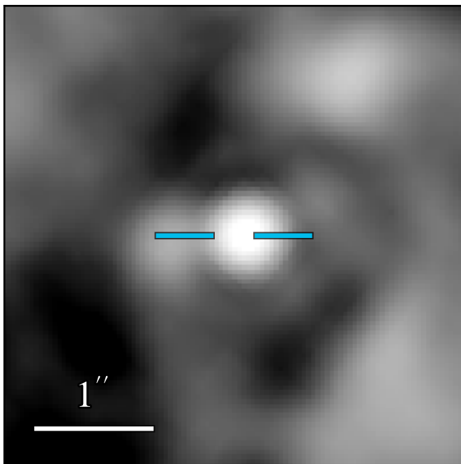
JWST/MIRI F1280W
