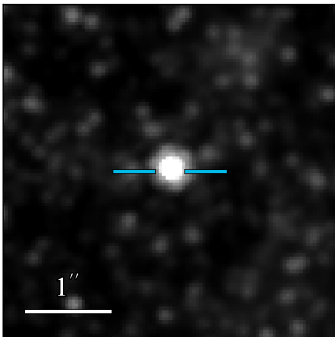
JWST/NIRCam F360M
