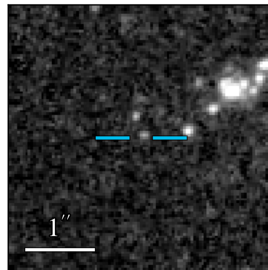
WFC3 F336W 24.944 \pm 0.123
