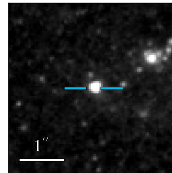
WFC3 F606W 21.229 \pm 0.003
