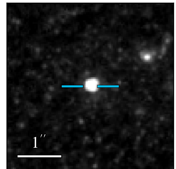
WFC3 F814W 19.765 \pm 0.003
