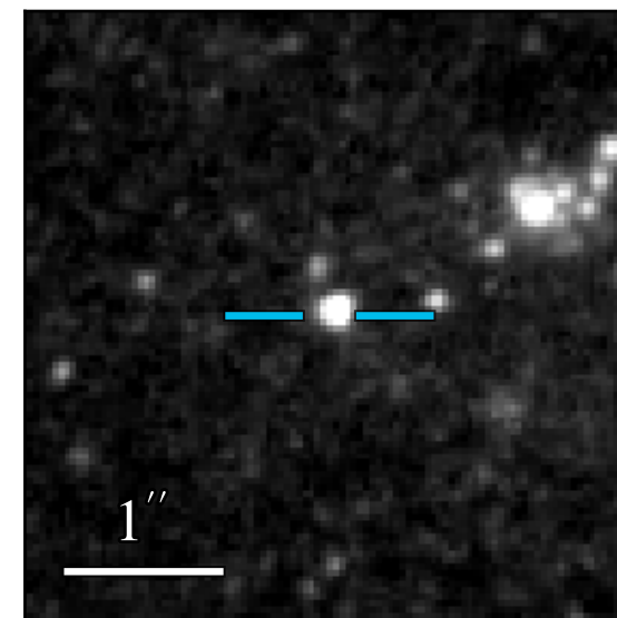
WFC3 F475W 22.536 \pm 0.007
