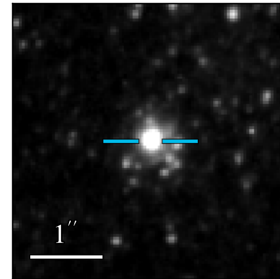
WFC3 F606W 21.311 \pm 0.018
