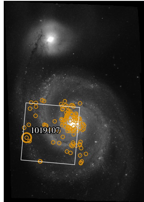
M51 / WFC3 footprint
