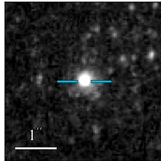
WFC3 F336W 21.476 \pm 0.027
