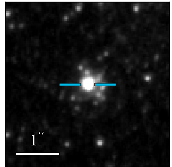
WFC3 F814W 20.924 \pm 0.030
