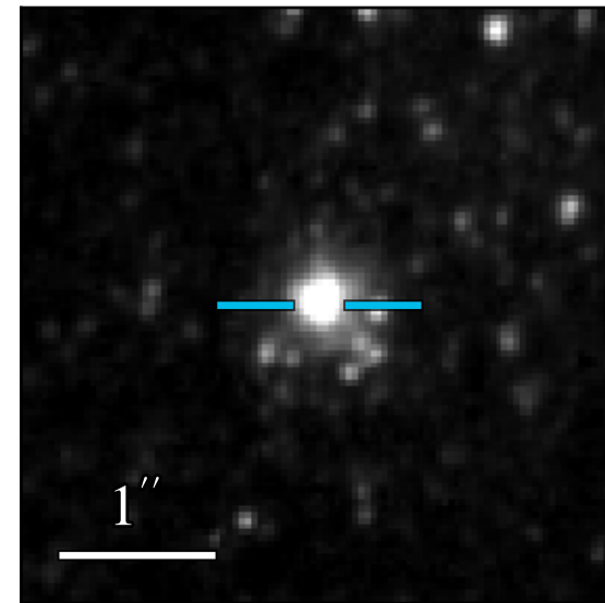
WFC3 F475W 21.561 \pm 0.016
