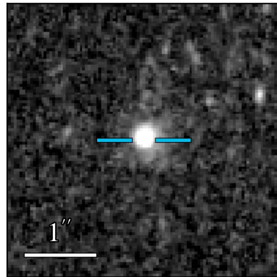
WFC3 F275W 21.513 \pm 0.036
