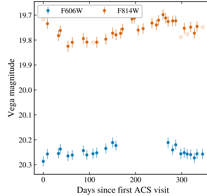
ACS visit light curves
