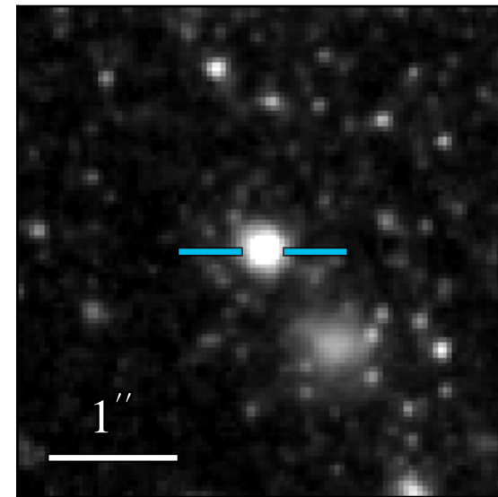
WFC3 F475W 21.413 \pm 0.007
