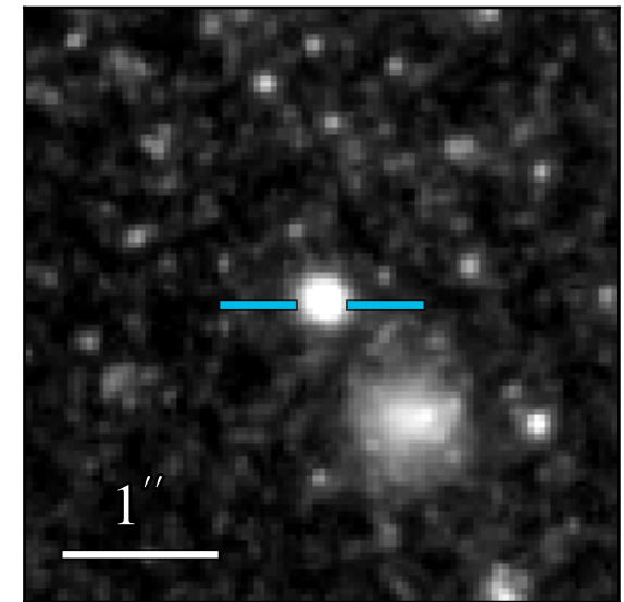
WFC3 F814W 20.701 \pm 0.008
