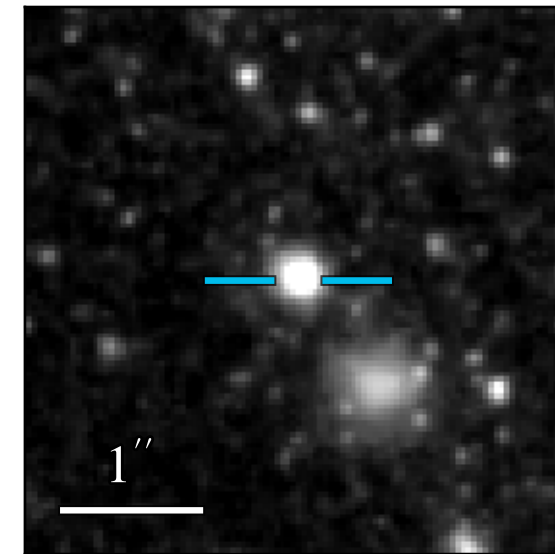
WFC3 F606W 21.240 \pm 0.007
