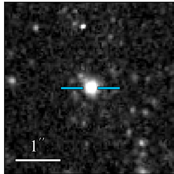
WFC3 F275W 20.213 \pm 0.012
