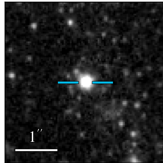
WFC3 F336W 20.458 \pm 0.010
