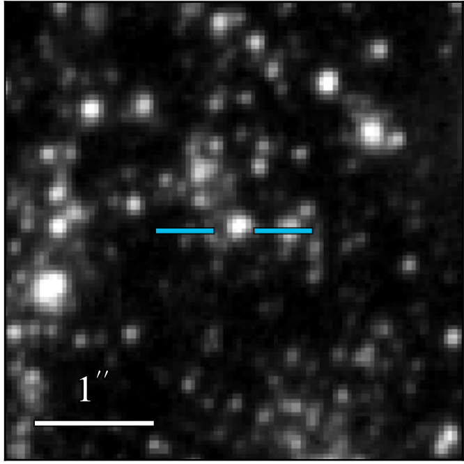
WFC3 F275W 20.834 ± 0.024
