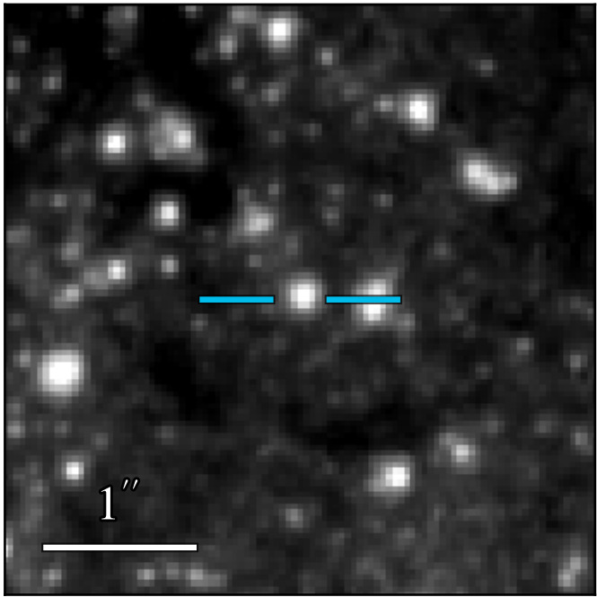
WFC3 F814W 20.994 ± 0.008
