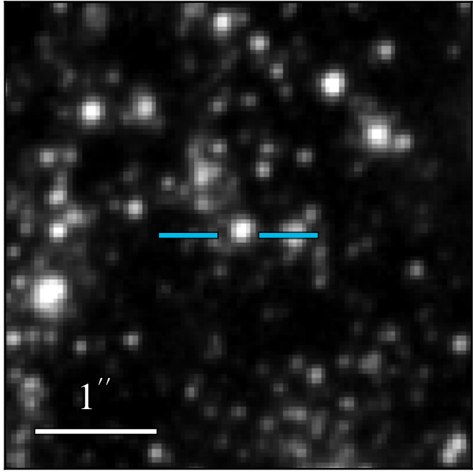
WFC3 F336W 20.926 ± 0.017
