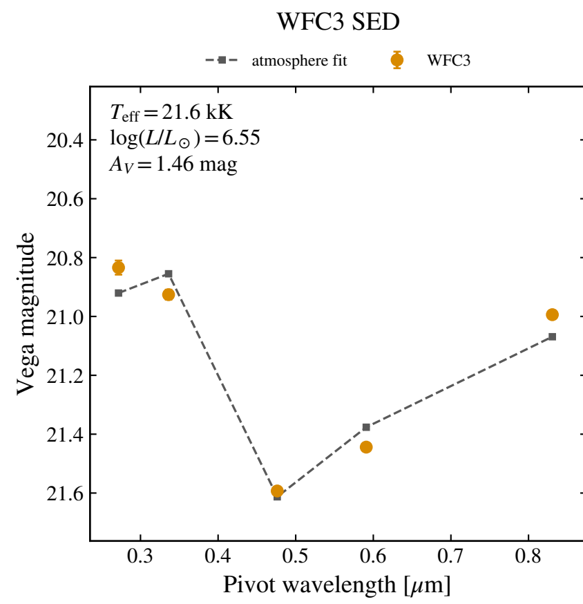
WFC3 F606W 21.444 ± 0.008
