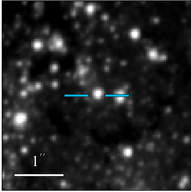
WFC3 F606W 21.444 ± 0.008
