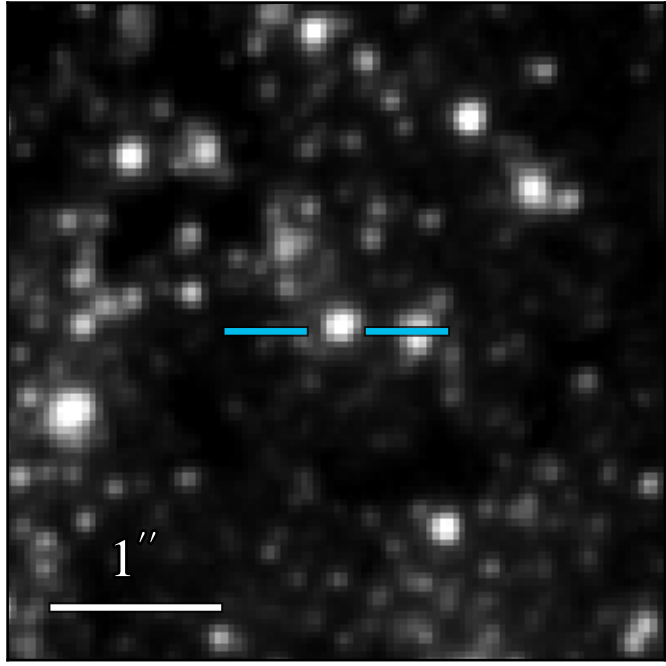
WFC3 F475W 21.593 ± 0.009
