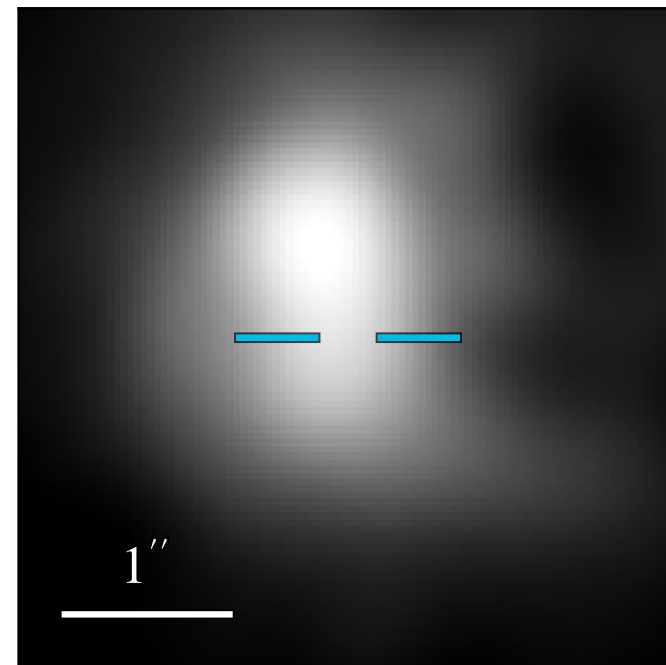
JWST/MIRI F1800W
