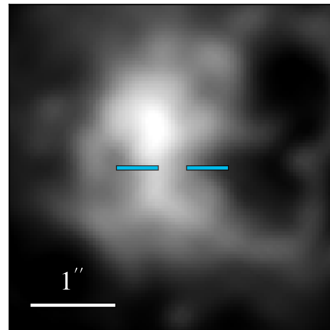
JWST/MIRI F770W
