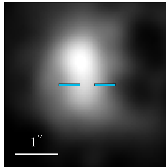
JWST/MIRI F1500W
