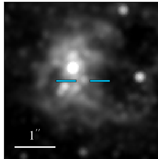
JWST/NIRCam F430M
