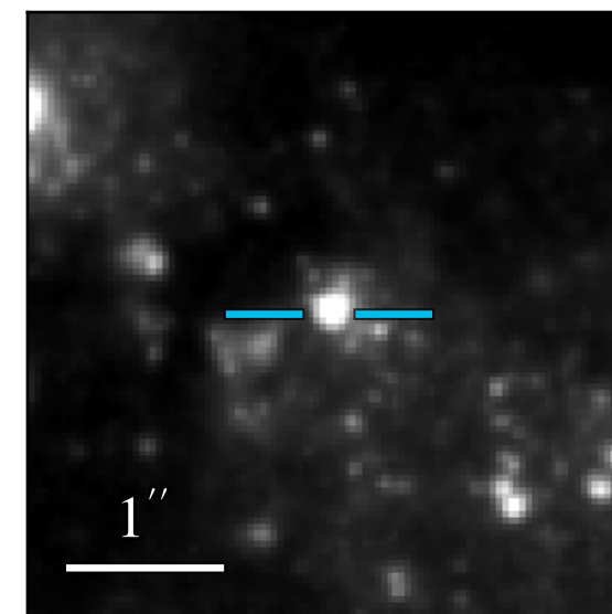
WFC3 F606W 20.204 \pm 0.004
