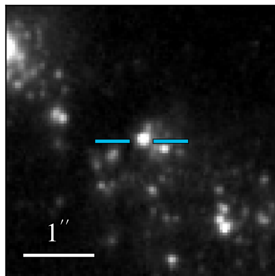
WFC3 F336W 20.692 \pm 0.010
