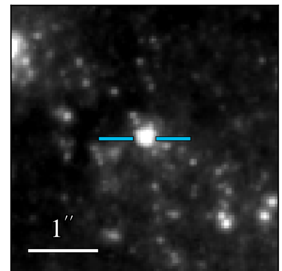
WFC3 F814W 19.485 \pm 0.004
