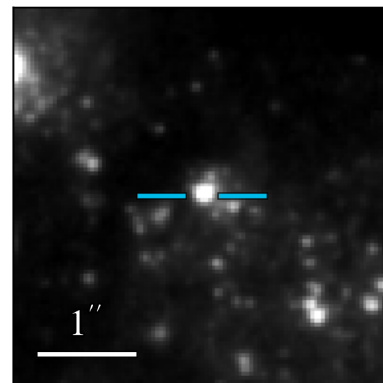
WFC3 F475W 20.851 \pm 0.005
