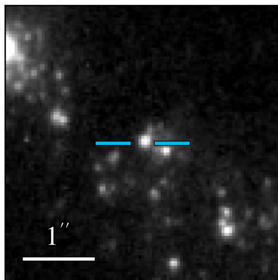
WFC3 F275W 21.289 \pm 0.020
